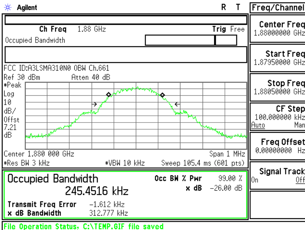
Plot 6-1. Occupied Bandwidth Plot (GSM1900 Mode - Ch.661)
