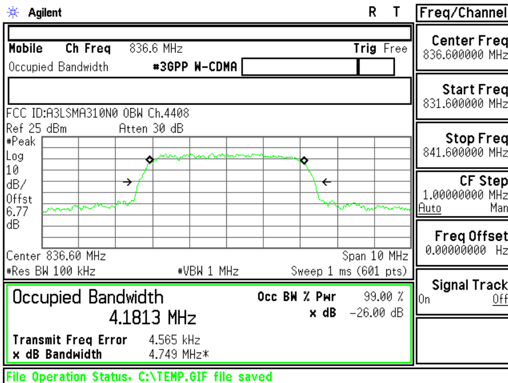
Plot 6-2. Occupied Bandwidth Plot (Cellular WCDMA Mode - Ch.4183(DL4408))
