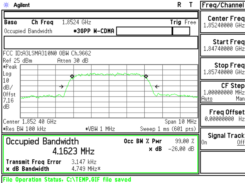
Plot 6-3. Occupied Bandwidth Plot (PCS WCDMA Mode - Ch.9262(DL9662))
