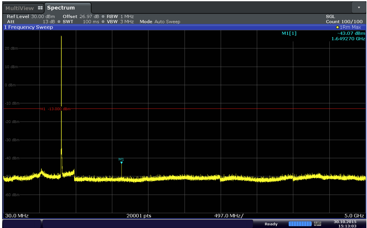
Plot 6-9. Conducted Spurious Plot (Band 5-1.4MHz-QPSK-RB Size 1-RB Offset 2-Ch.20407)
