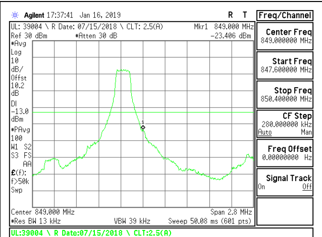
LTE B5 1.4MHz QPSK High Channel RB1-5
