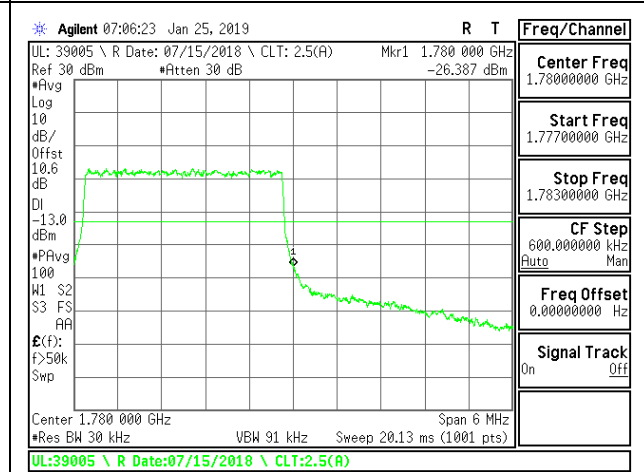
LTE B66 3MHz 16QAM High Channel RB15-0
