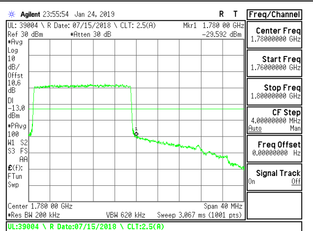
LTE B66 20MHz QPSK High Channel RB100-0
