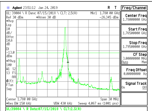
LTE B66 15MHz 16QAM High Channel RB1-74
