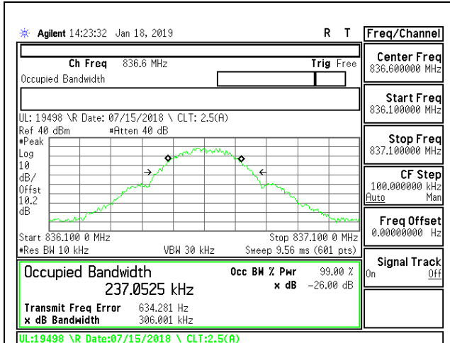
GSM 850MHz GPRS MID Channel
