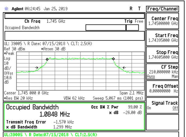
LTE B66 1.4MHz 16QAM Mid Channel RB6-0
