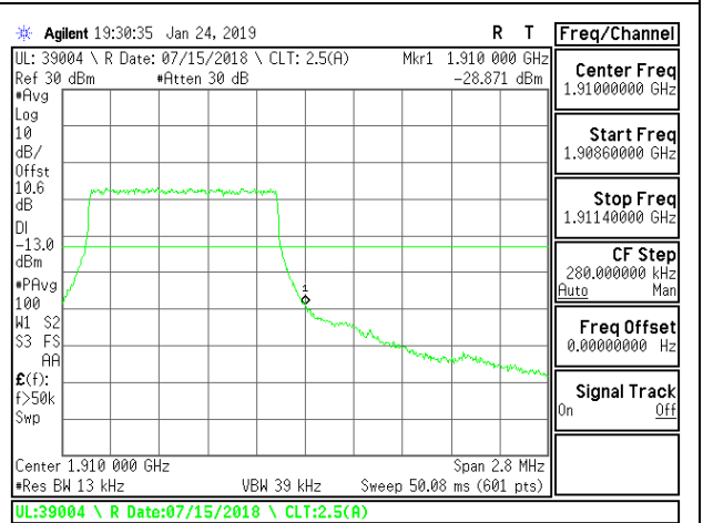
LTE B2 1.4MHz QPSK High Channel RB6-0
