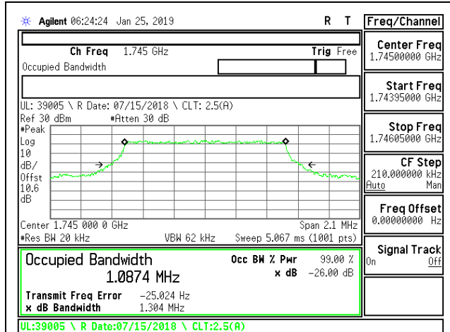
LTE B66 1.4MHz QPSK Mid Channel RB6-0
