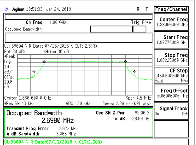
LTE B2 3MHz 16QAM Mid Channel RB15-0
