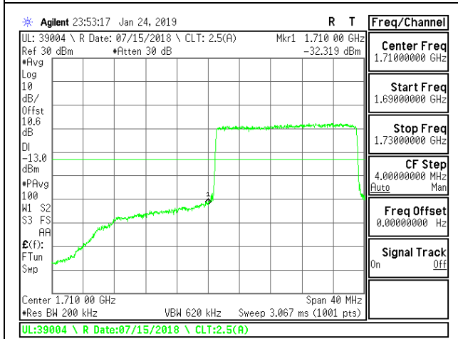
LTE B66 20MHz QPSK Low Channel RB100-0
