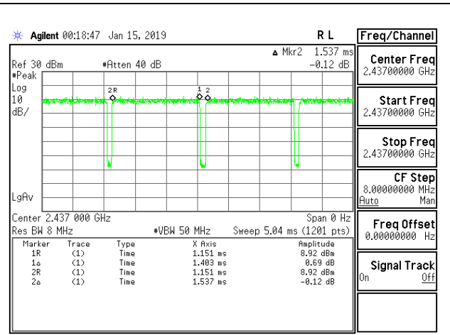
DUTY CYCLE 802.11g MODE
