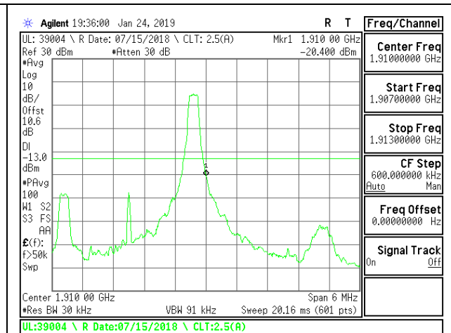
LTE B2 3MHz 16QAM High Channel RB1-14
