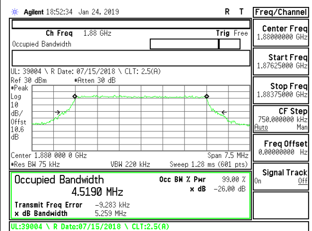
LTE B2 5MHz 16QAM Mid Channel RB25-0
