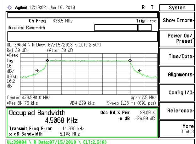
LTE B5 5MHz 16QAM Mid Channel RB25-0
