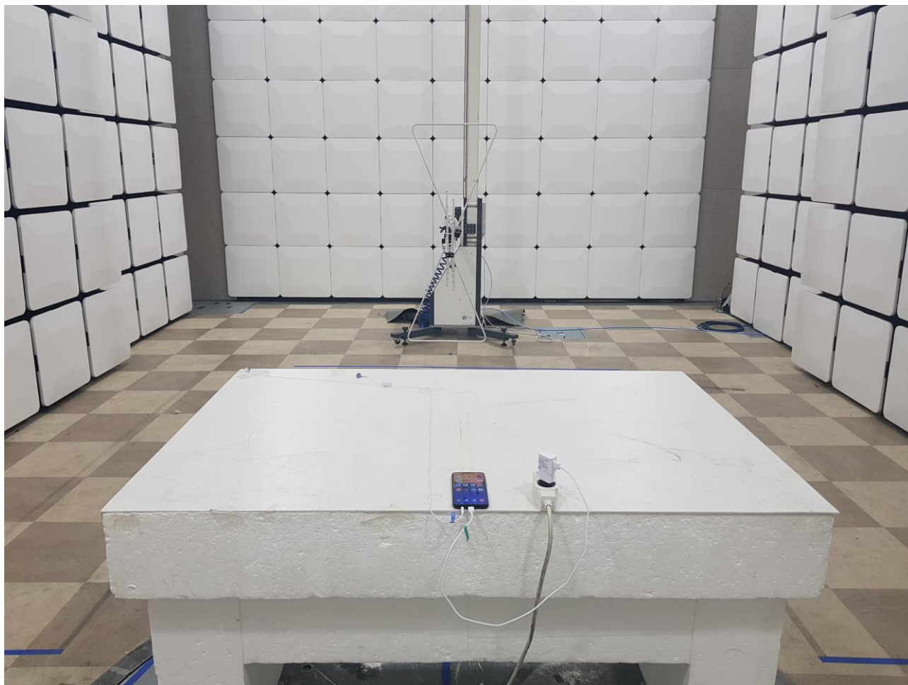
RE_ Rear
