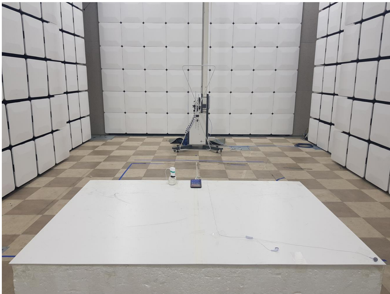
RE_ Front
