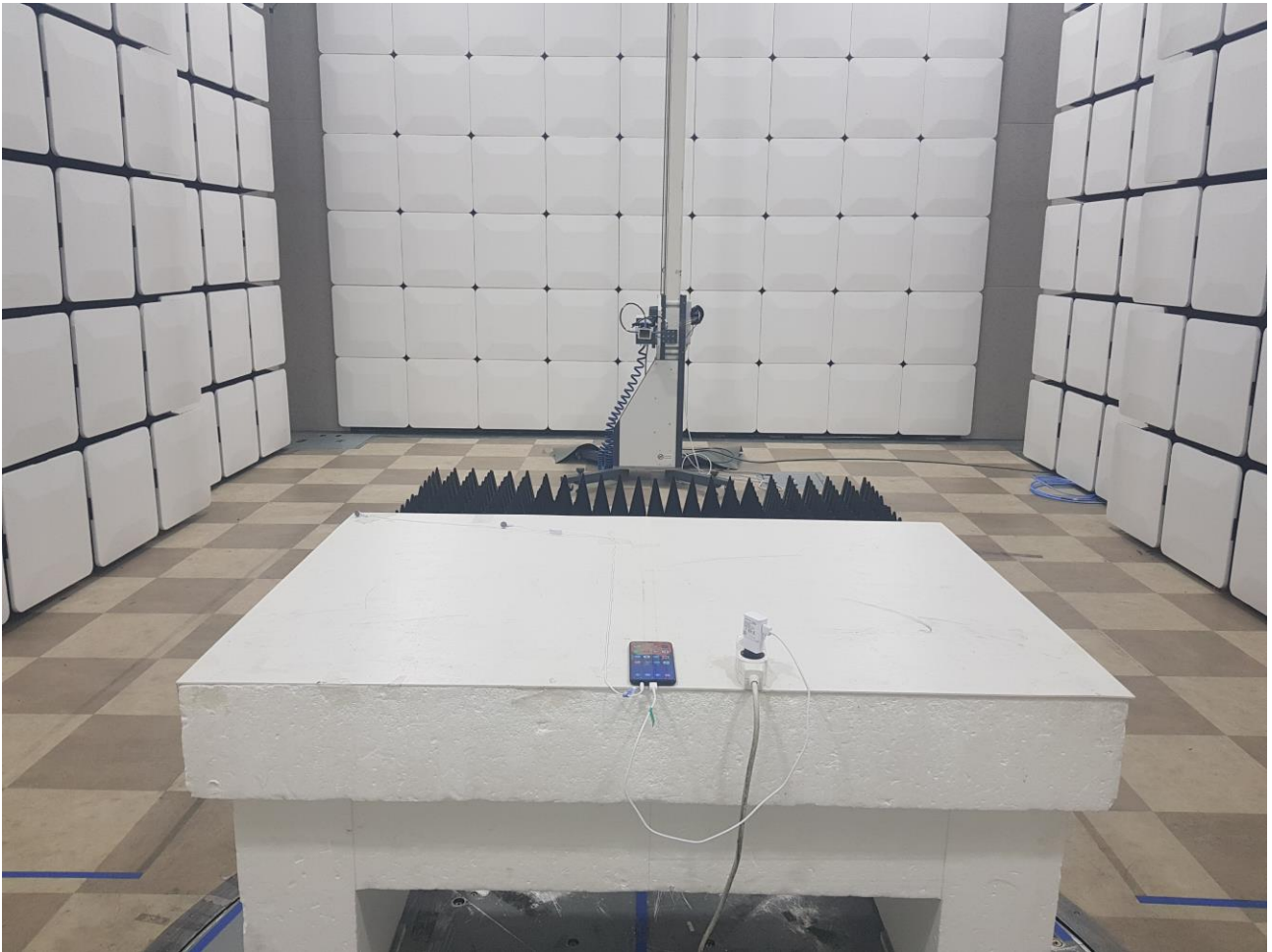
RE_18~30GHz_ Rear
