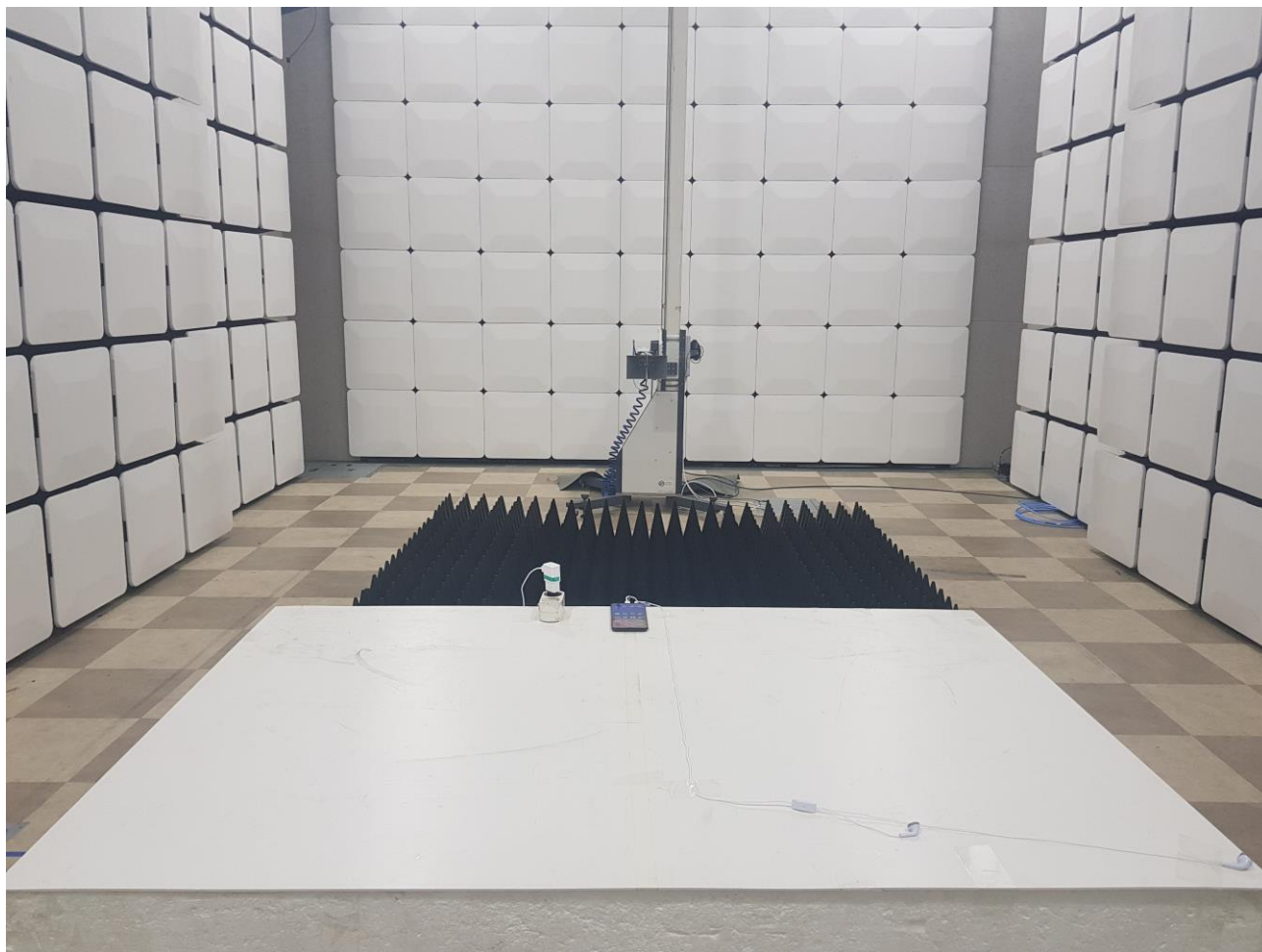
RE_1~18GHz_ Front
