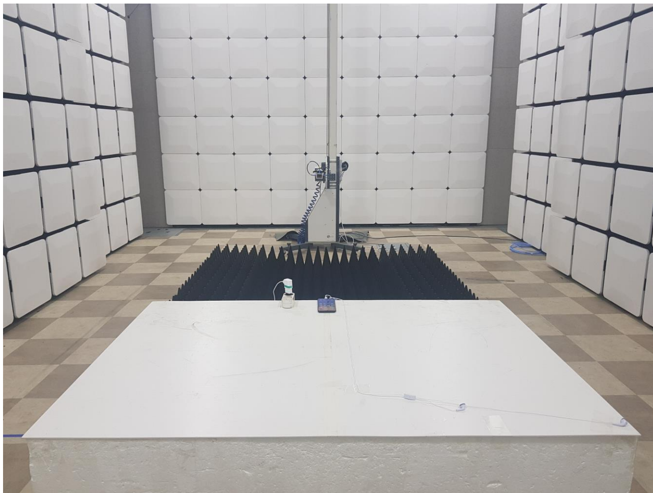
RE_18~30GHz_ Front
