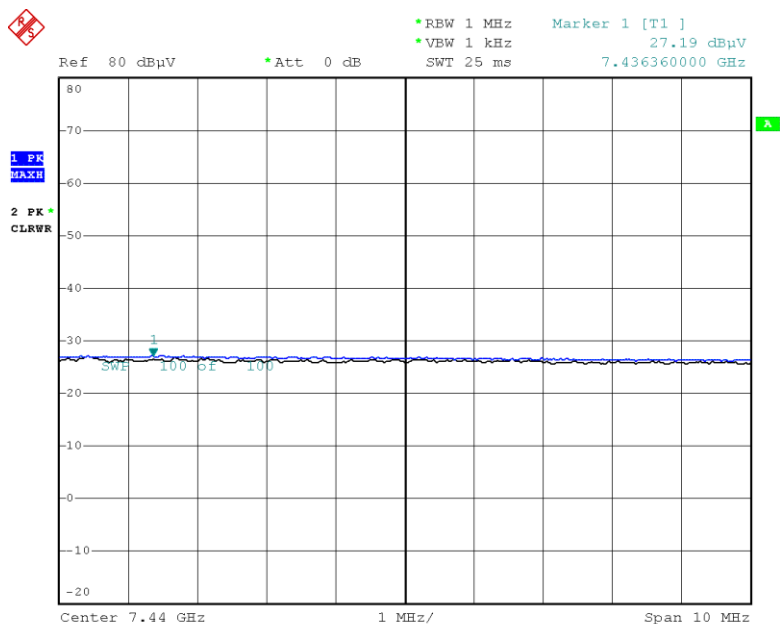
Radiated Spurious Emissions plot – Average Reading (8DPSK, Ch.78 3rd Harmonic)
