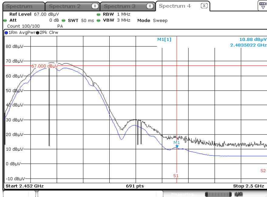
Radiated Restricted Band Edges plot – Average Result (802.11b_1 Mbps, Ch.11, X-H)
