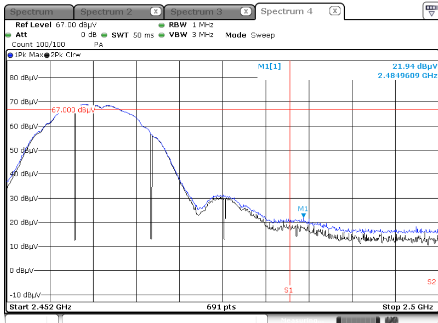
Radiated Restricted Band Edges plot – Peak Result (802.11b_1 Mbps, Ch.11, X-H)
