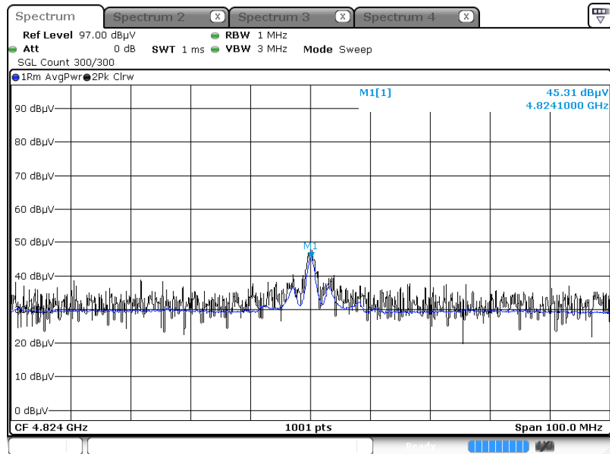
Radiated Spurious Emissions plot – Average Result (802.11b_1 Mbps, Ch.1 2nd Harmonic, X-H)
