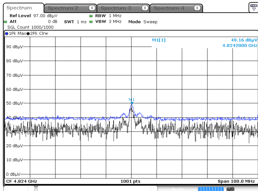
Radiated Spurious Emissions plot – Peak Result (802.11b_1 Mbps, Ch.1 2nd Harmonic, X-H)
