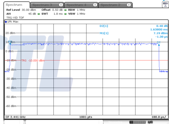
2-DH3
