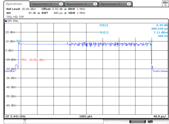
2-DH1
