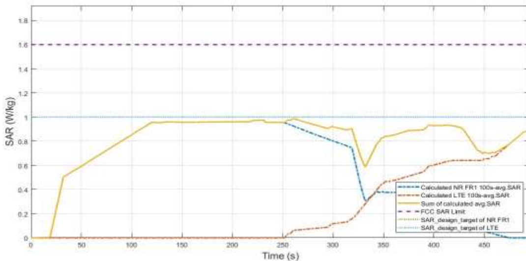
Figure 7.6-4 Total time-averaged SAR in TC07
