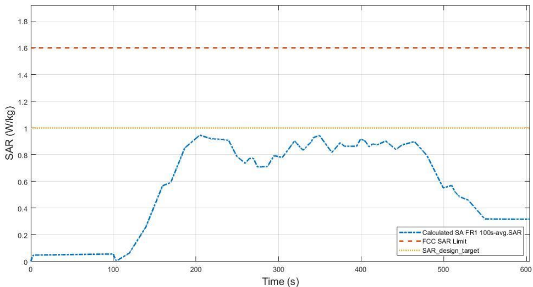
Figure 7.3-22 Total time-averaged SAR in TC04
