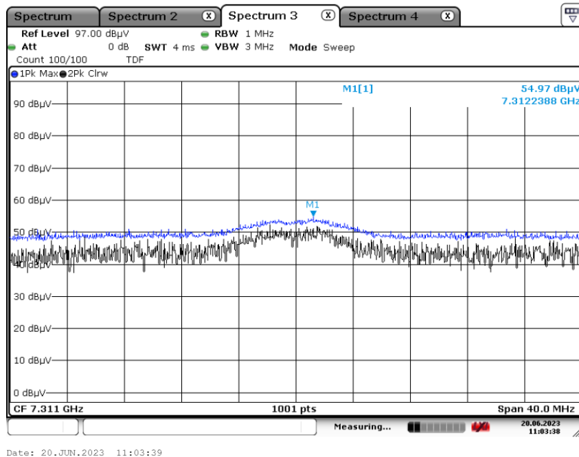
Radiated Spurious Emissions plot – Peak Result (802.11b_1 Mbps, Ch.6 3rd Harmonic)
