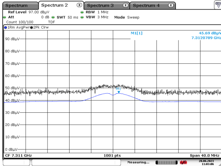
Radiated Spurious Emissions plot – Average Result (802.11b_1 Mbps, Ch.6 3rd Harmonic)
