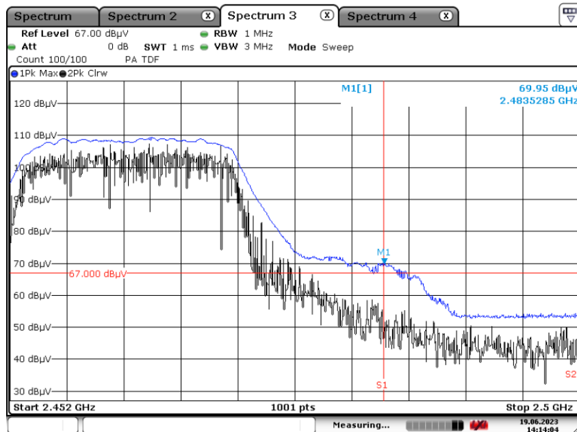
Radiated Restricted Band Edges plot – Peak Result (802.11n (HT20), 6 Mbps, Ch.11, X-H)
