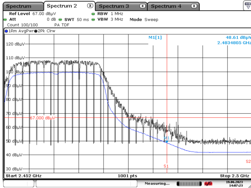
Radiated Restricted Band Edges plot – Average Result (802.11n (HT20), 6 Mbps, Ch.11, X-H)
