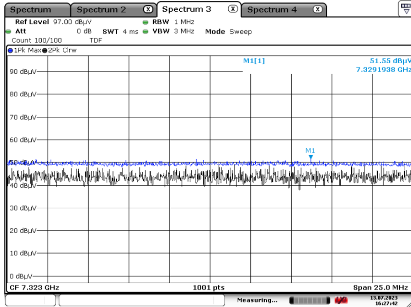
Radiated Spurious Emissions plot – Average & Peak Result (Restricted Harmonic, H)
