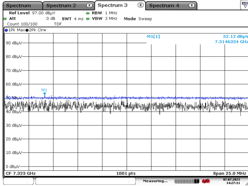
Radiated Spurious Emissions plot – Average & Peak Result (GFSK, Ch.39 3 rd Harmonic, H)
