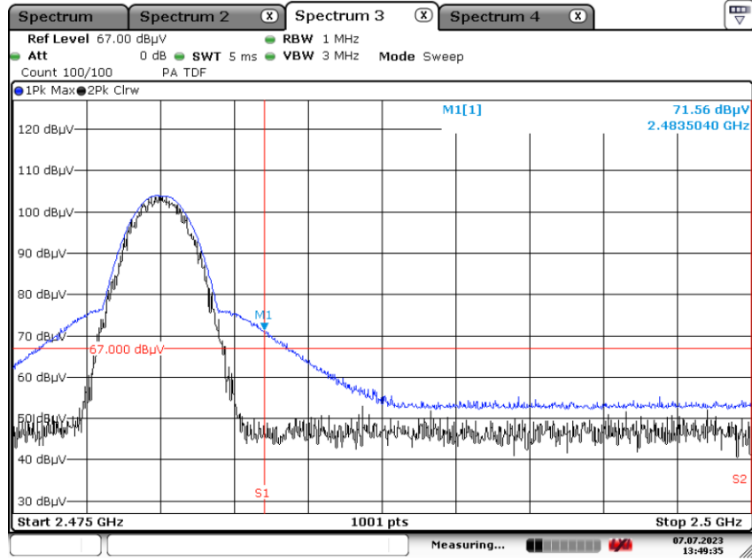
Radiated Restricted Band Edges plot – Average & Peak Result ( \pi/4 DQPSK, Ch.78, H)
