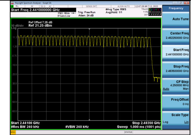
8DPSK Number of Channels (2.441 GHz - 2.483.5 GHz)
