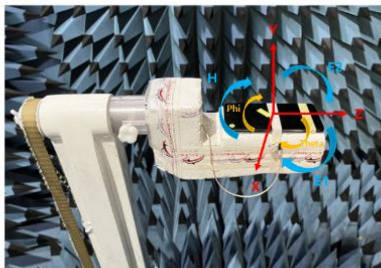
Geometry for SM-A256U for Radiation patterns.
