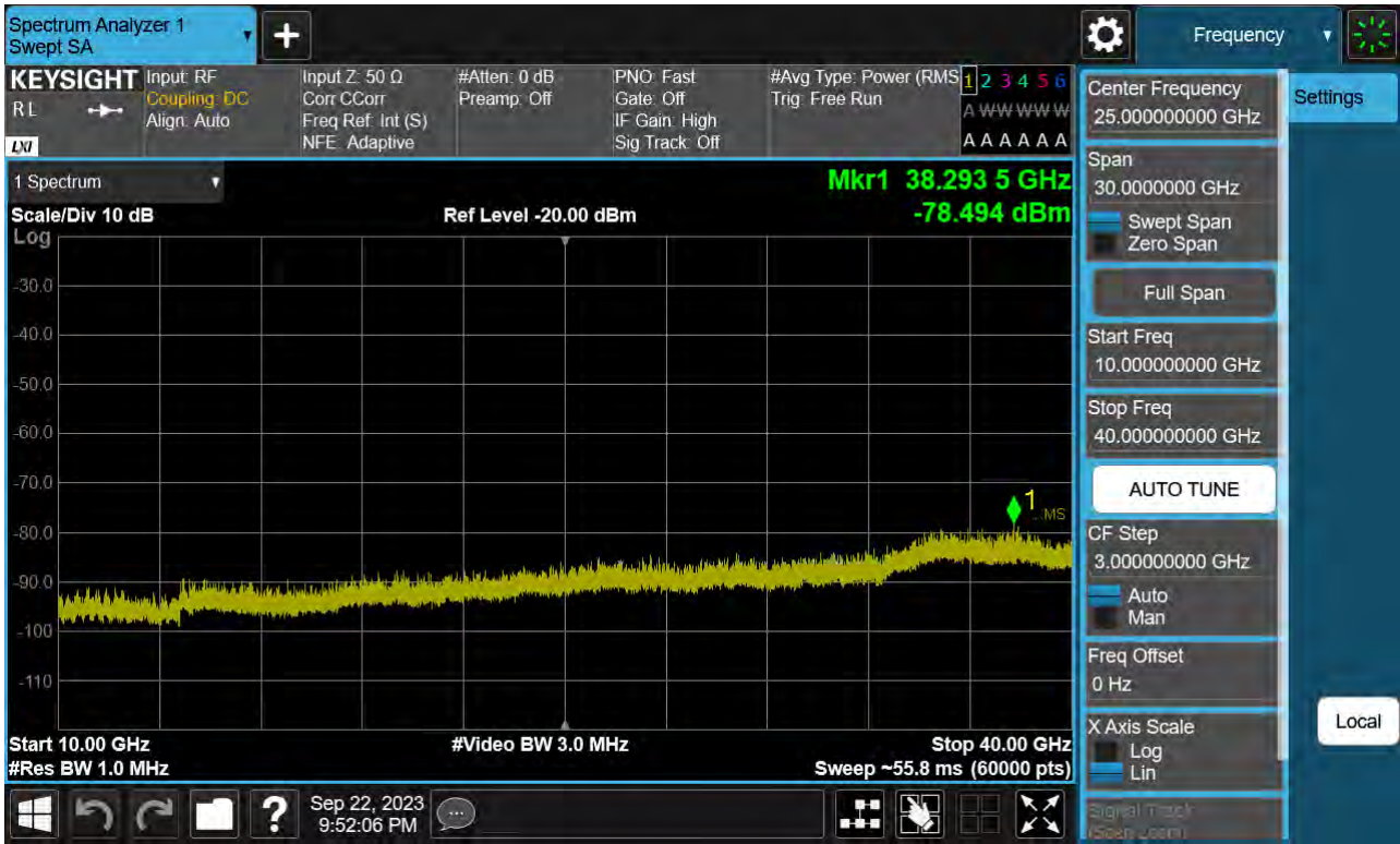
Sub6 n77. Conducted Spurious Plot_2 (664500ch_25 MHz_BPSK)
