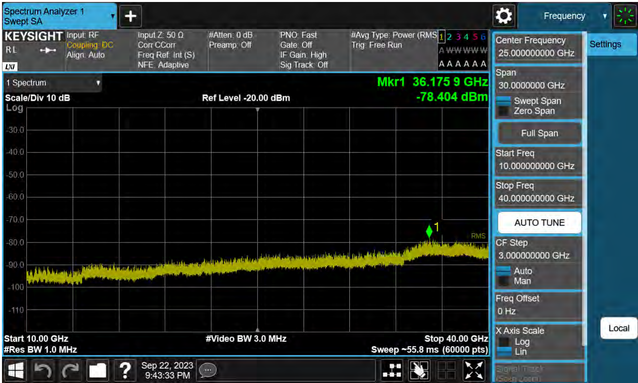
Sub6 n77. Conducted Spurious Plot_2 (647500ch_25 MHz_BPSK)
