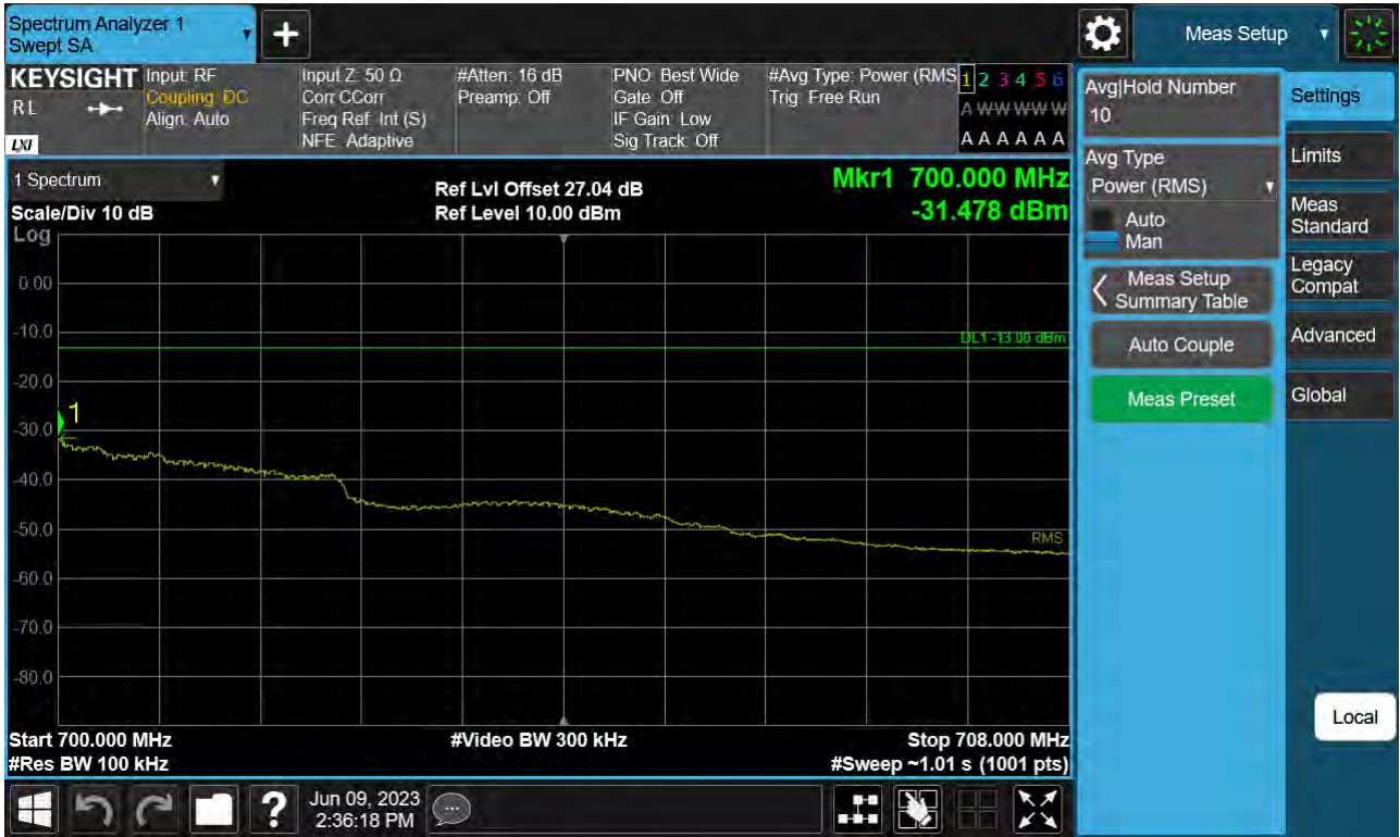
Sub6 n71. Upper Extended Band Edge Plot (5 M BW Ch.139100 BPSK_ Full RB)
