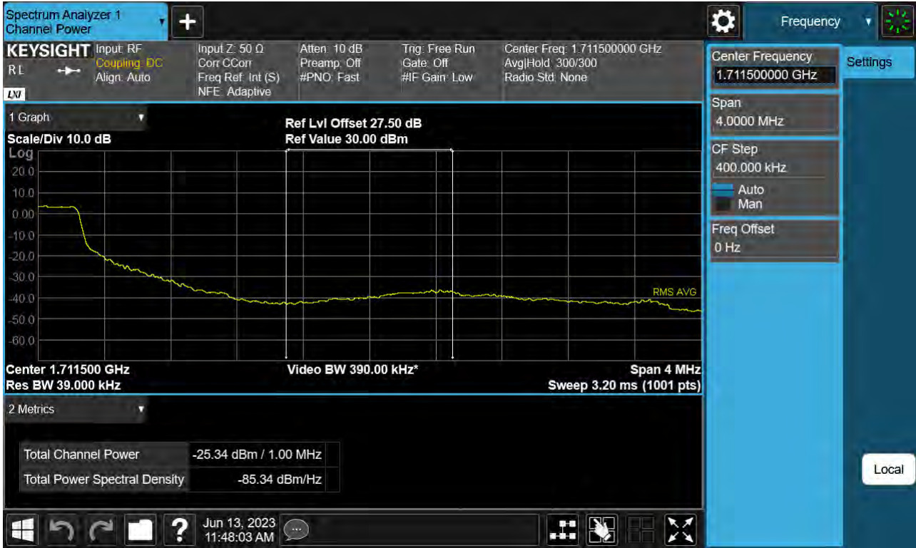
Sub6 n70. Upper Extended Band Edge Plot (5 M BW Ch.341500 BPSK_ Full RB) -3
