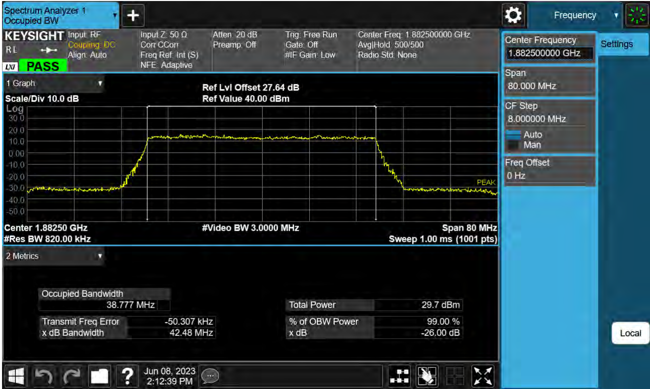
Sub6 n25(2). Occupied Bandwidth Plot (40 M BW Ch.376500 BPSK_ Full RB_0)
