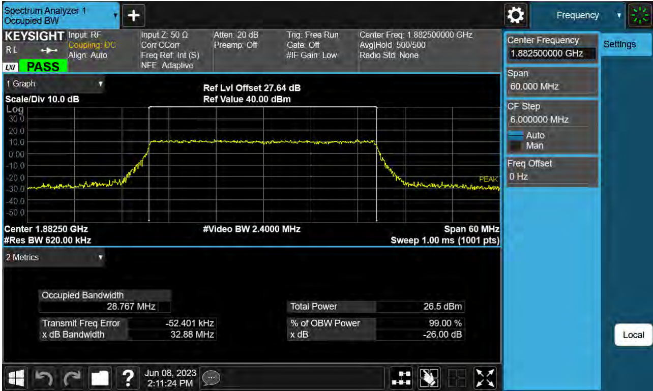
Sub6 n25(2). Occupied Bandwidth Plot (30 M BW Ch.376500 64QAM_ Full RB_0 )
