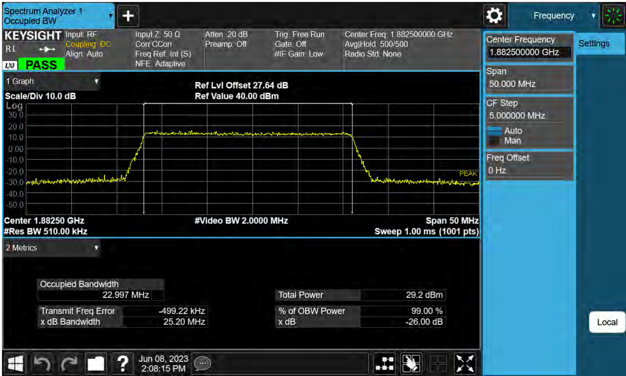
Sub6 n25(2). Occupied Bandwidth Plot (25 M BW Ch.376500 QPSK _ Full RB _0)
