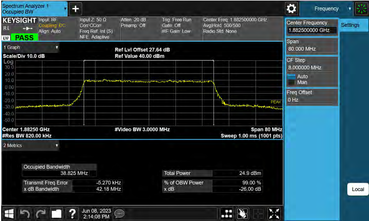
Sub6 n25(2). Occupied Bandwidth Plot (40 M BW Ch.376500 256QAM_ Full RB _0 )
