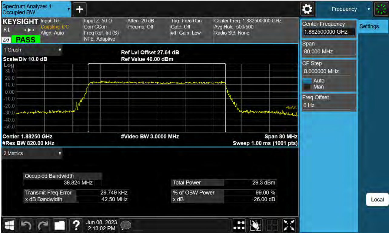
Sub6 n25(2). Occupied Bandwidth Plot (40 M BW Ch.376500 QPSK_ Full RB _0)
