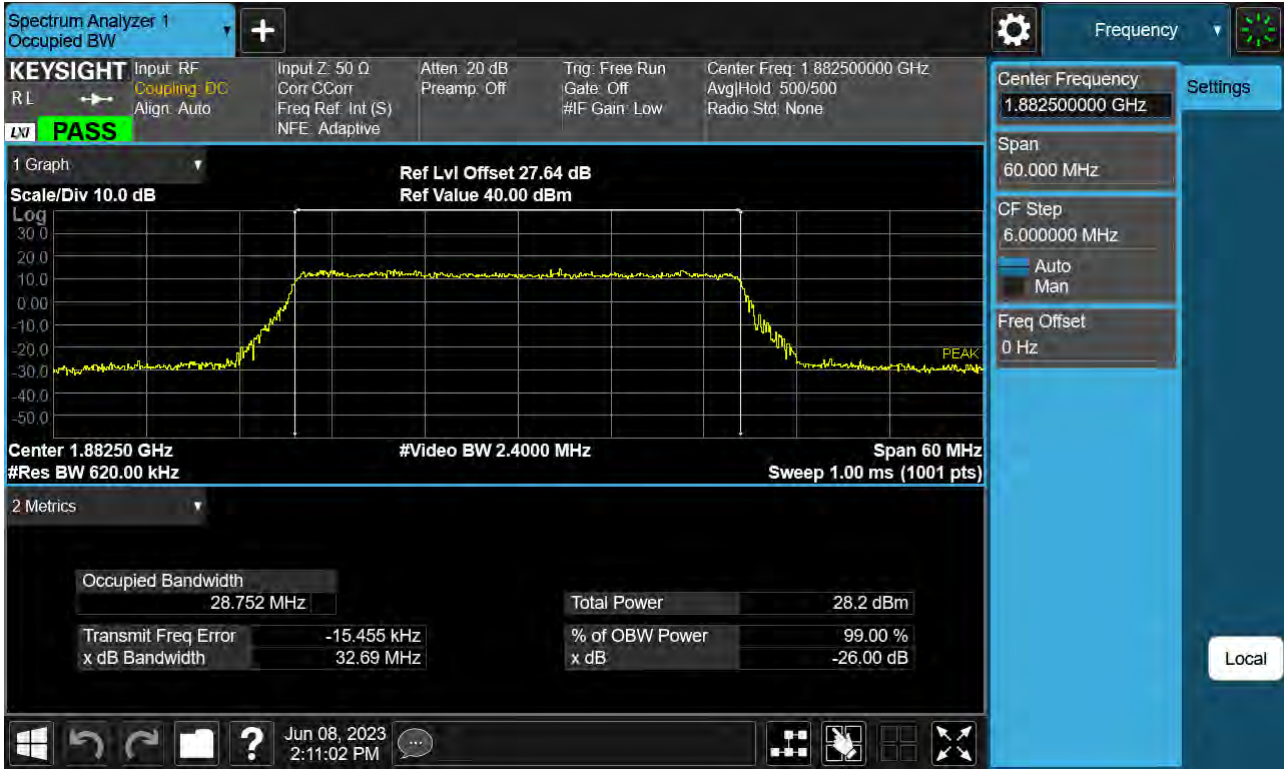
Sub6 n25(2). Occupied Bandwidth Plot (30 M BW Ch.376500 16QAM _ Full RB _0)
