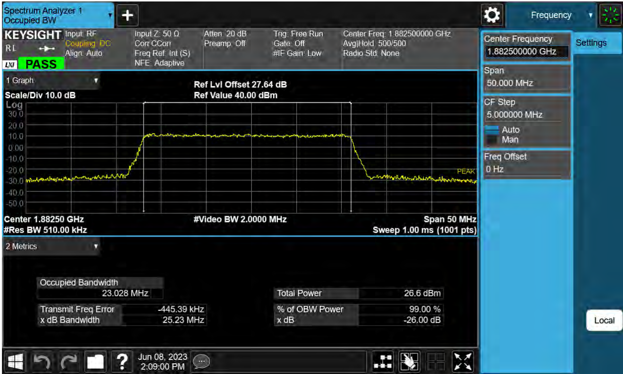
Sub6 n25(2). Occupied Bandwidth Plot (25 M BW Ch.376500 64QAM _ Full RB _0)
