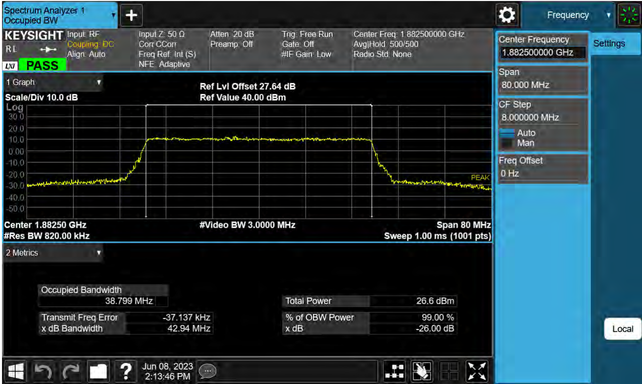
Sub6 n25(2). Occupied Bandwidth Plot (40 M BW Ch.376500 64QAM_ Full RB_0 )
