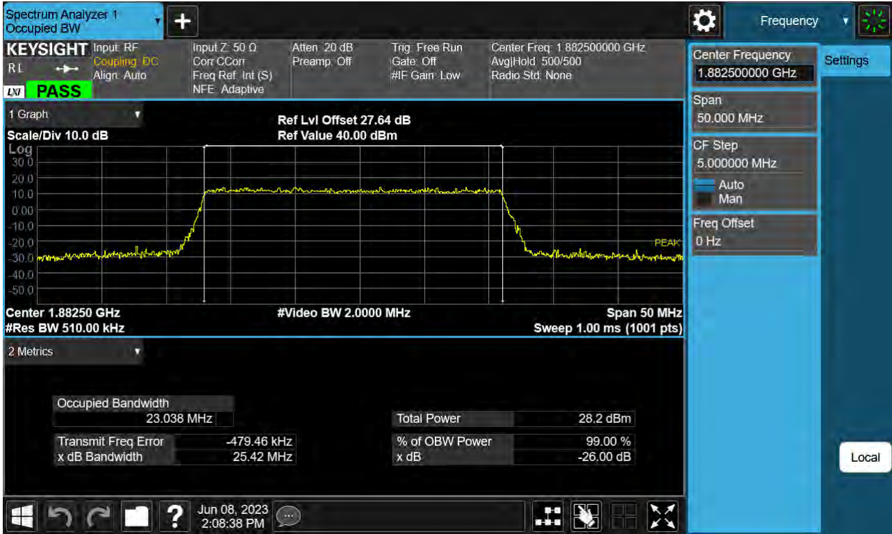
Sub6 n25(2). Occupied Bandwidth Plot (25 M BW Ch.376500 16QAM _ Full RB _0)
