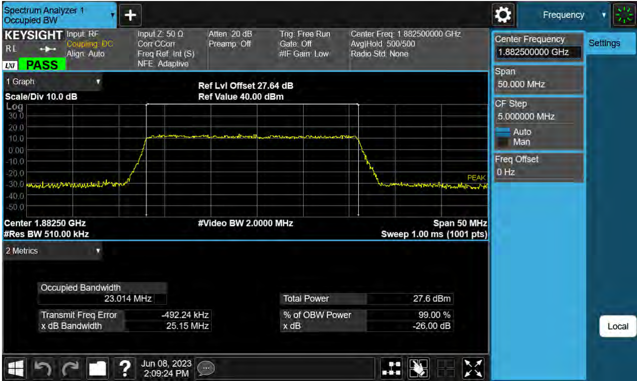
Sub6 n25(2). Occupied Bandwidth Plot (25 M BW Ch.376500 256QAM _ Full RB _0)
