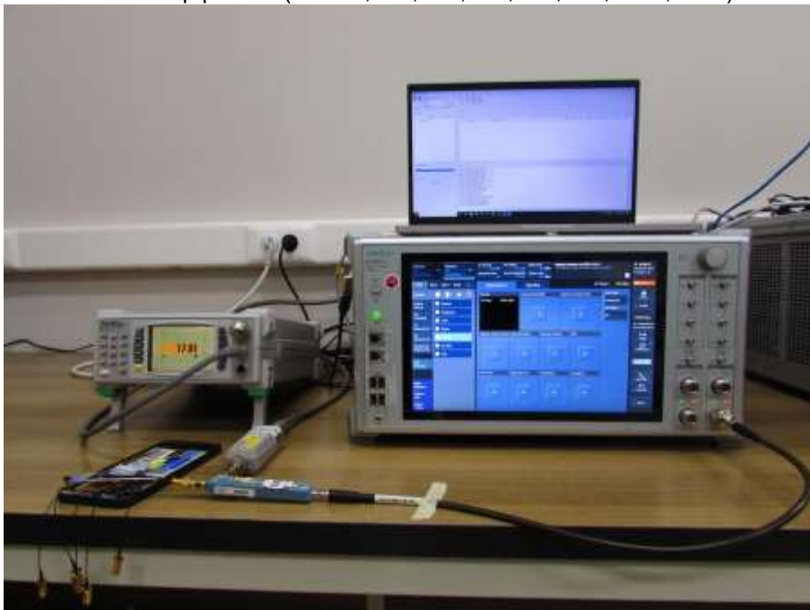
Test setup photo-2(TC 1-3, 3-3, 5-3)
