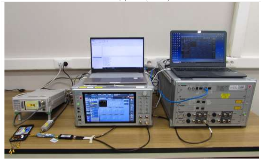
Test setup photo-6(TC 6-2)
