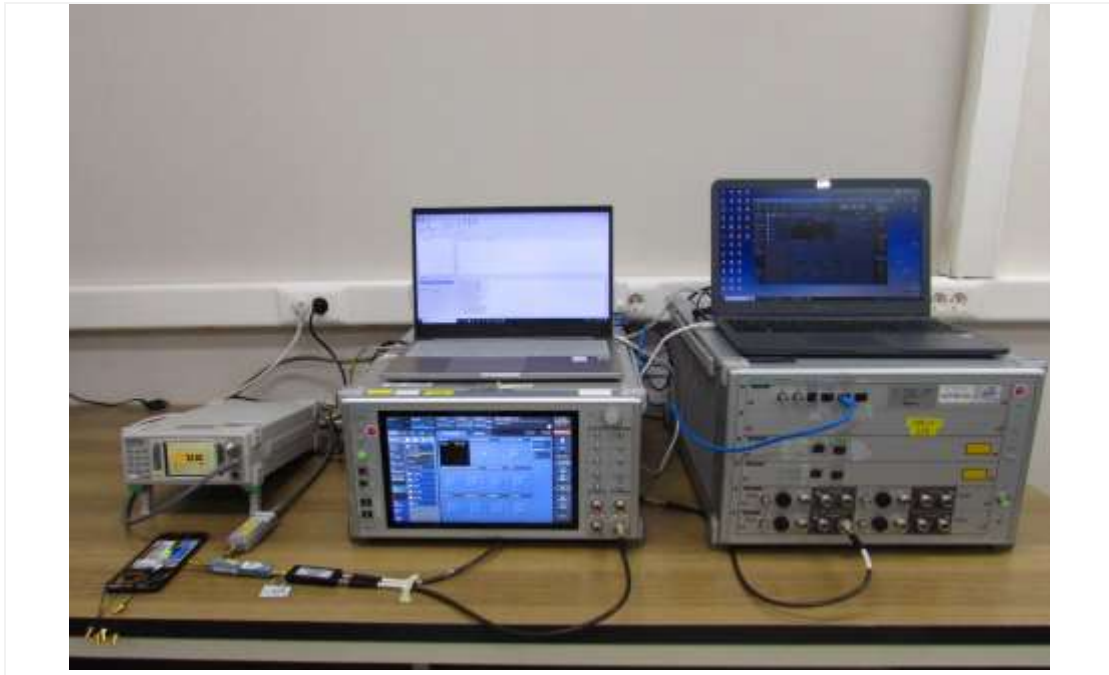
Test setup photo-5(TC 6-1)
