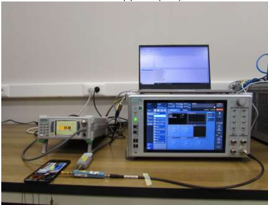
Test setup photo-10(TC 11-1, 11-2)
