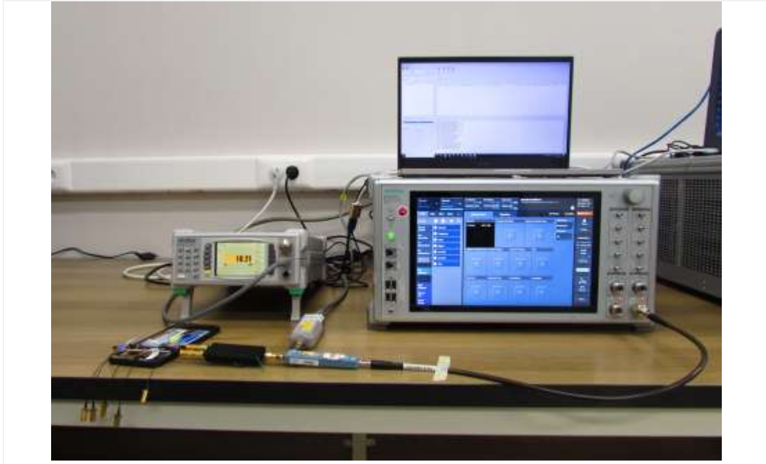
Test setup photo-11(TC 12-1)
