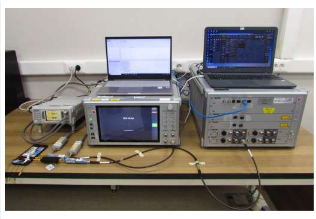
Test setup photo-15(TC 14)
