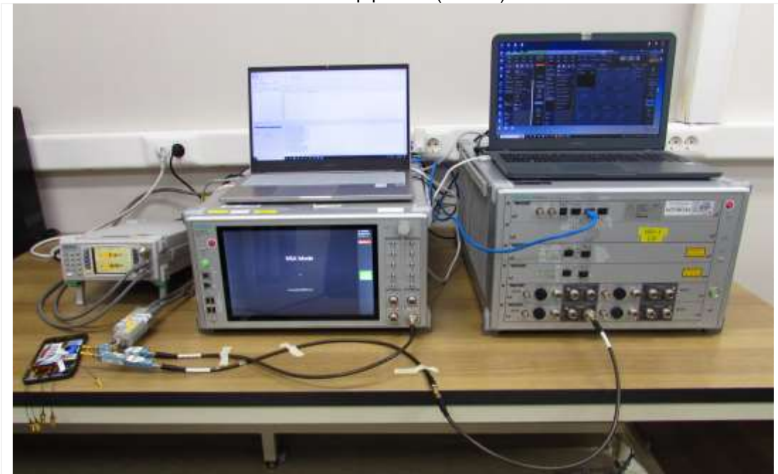
Test setup photo-8(TC 7-1, 7-2)
