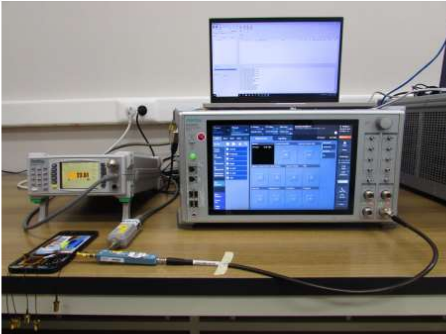
Test setup photo-1(TC 1-1, 1-2, 3-1, 3-2, 5-1, 5-2, 10-1, 10-2)
