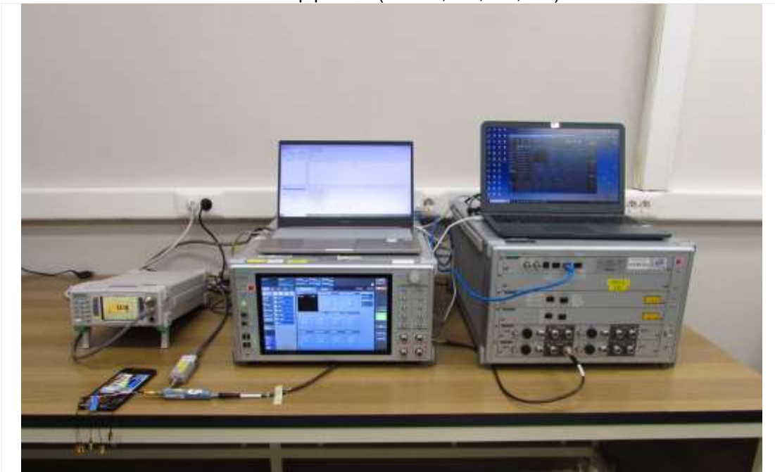
Test setup photo-4(TC 2-3, 4-3, 8)
