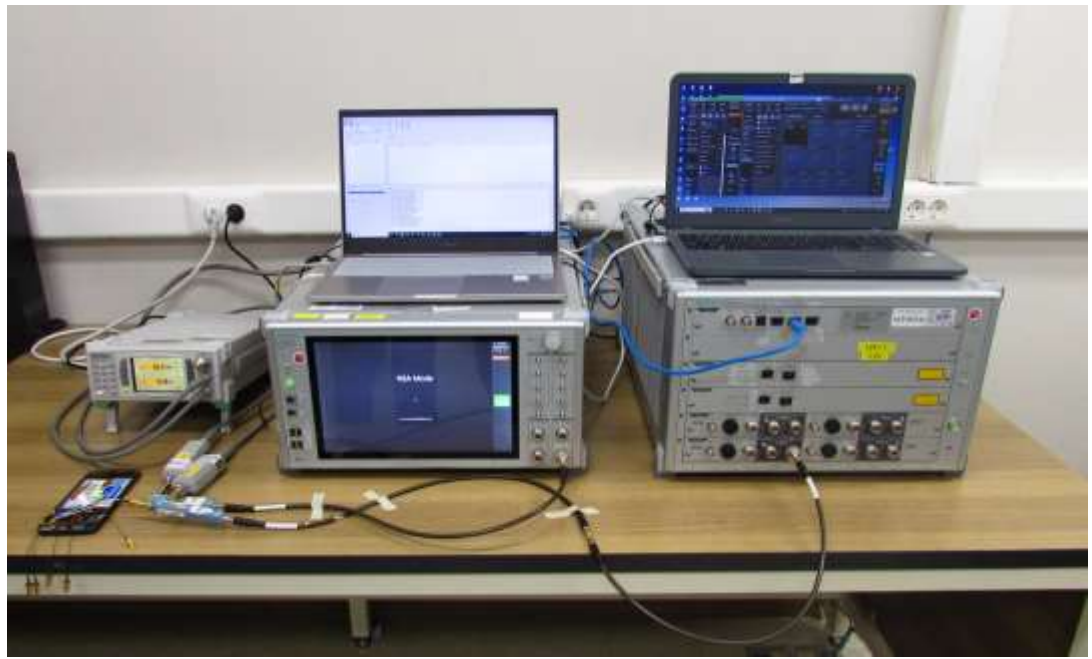
Test setup photo-13(TC 13-1)
