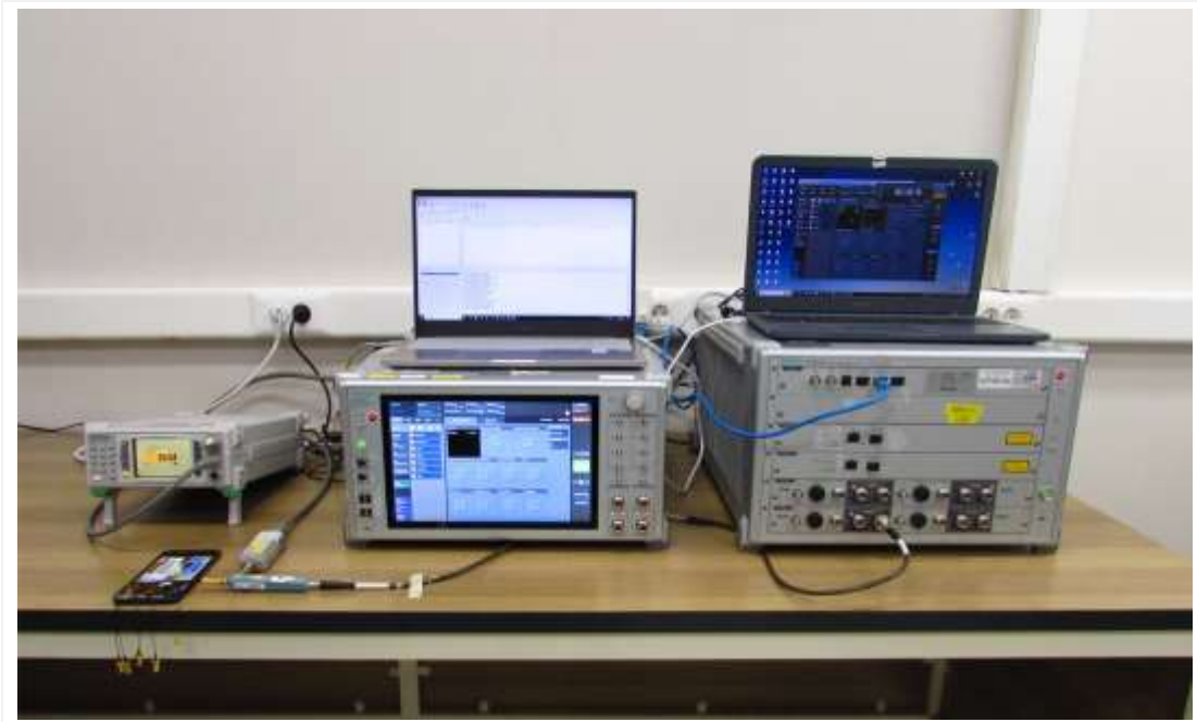
Test setup photo-3(TC 2-1, 2-2, 4-1, 4-2)
