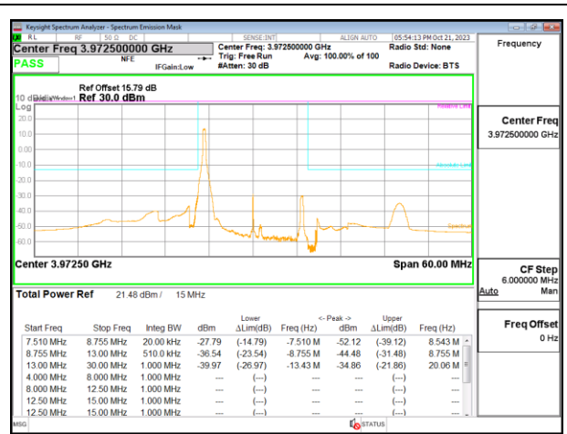
5G NR n77 15MHz QPSK High Channel RB1-0
