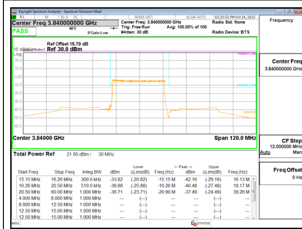
5G NR n77 30MHz QPSK Middle Channel RB75-0
