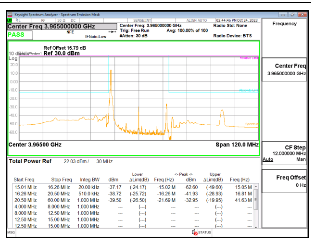
5G NR n77 30MHz QPSK High Channel RB1-0
