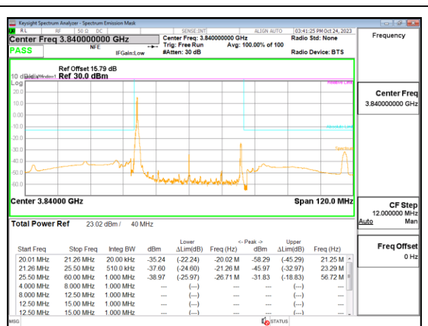
5G NR n77 40MHz QPSK Middle Channel RB1-0
