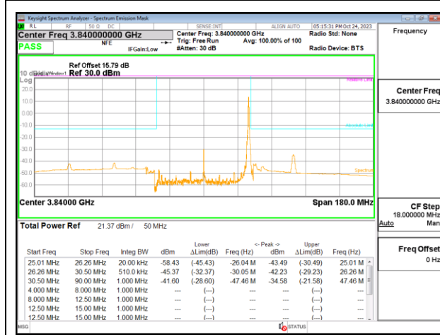
5G NR n77 50MHz QPSK Middle Channel RB1-132
