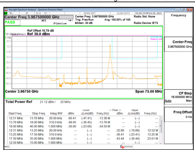
5G NR n77 25MHz QPSK High Channel RB1-64
