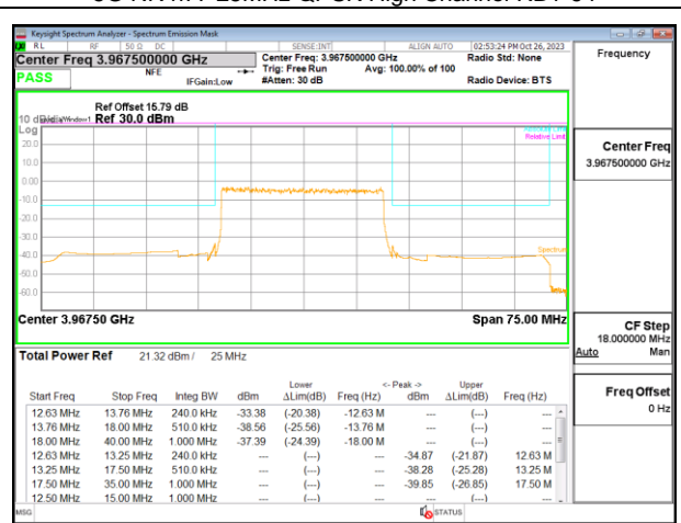
5G NR n77 25MHz QPSK High Channel RB64-0
