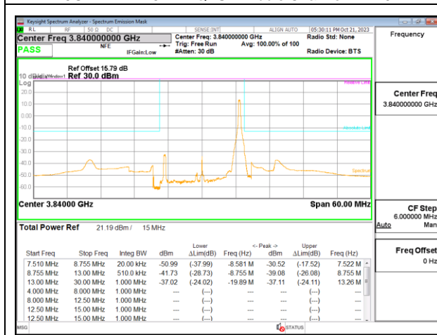
5G NR n77 15MHz QPSK Middle Channel RB1-37
