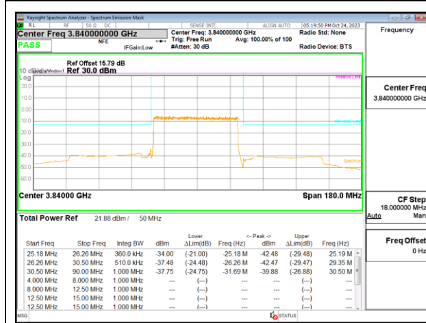
5G NR n77 50MHz QPSK Middle Channel RB128-0
