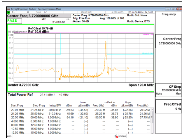
5G NR n77 40MHz QPSK Low Channel RB1-105
