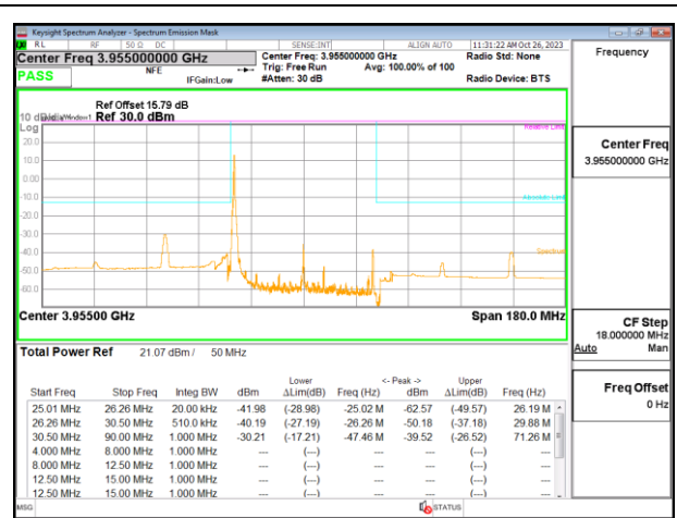
5G NR n77 50MHz QPSK High Channel RB1-0
