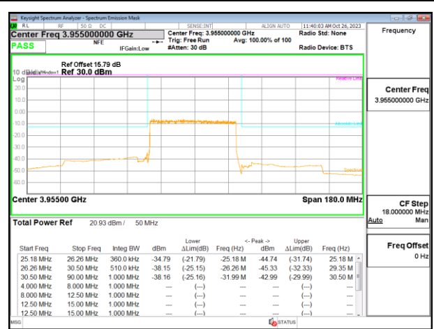
5G NR n77 50MHz QPSK High Channel RB128-0
