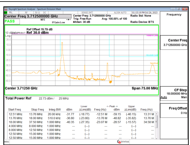
5G NR n77 25MHz QPSK Low Channel RB1-0
