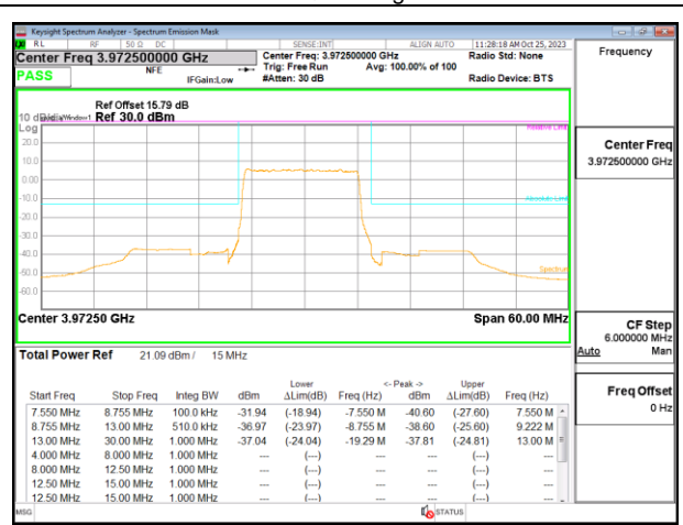
5G NR n77 15MHz QPSK High Channel RB36-0
