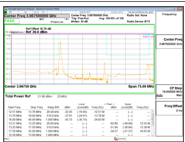
5G NR n77 25MHz QPSK High Channel RB1-0
