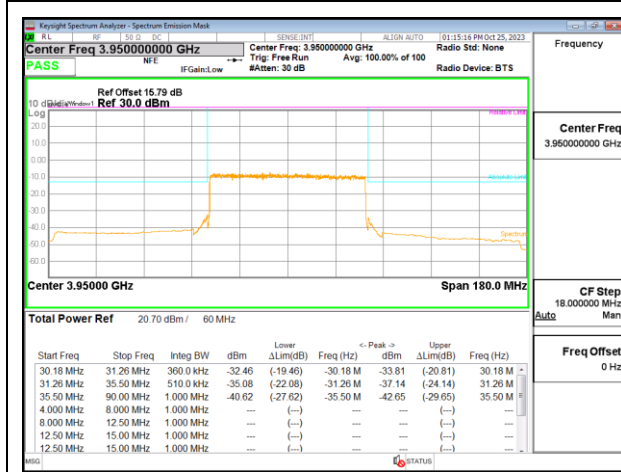
5G NR n77 60MHz QPSK High Channel RB162-0
