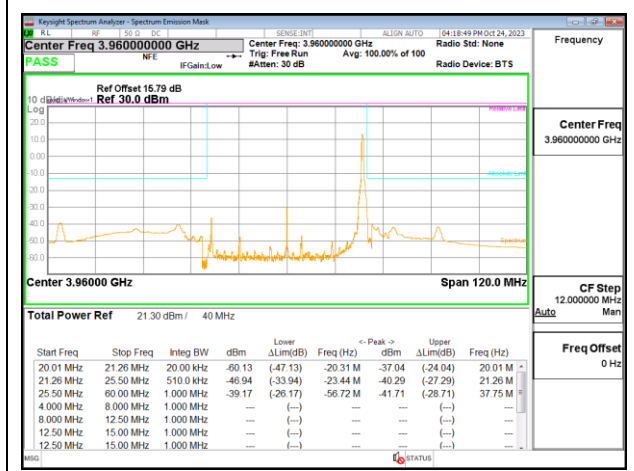
5G NR n77 40MHz QPSK High Channel RB1-105
