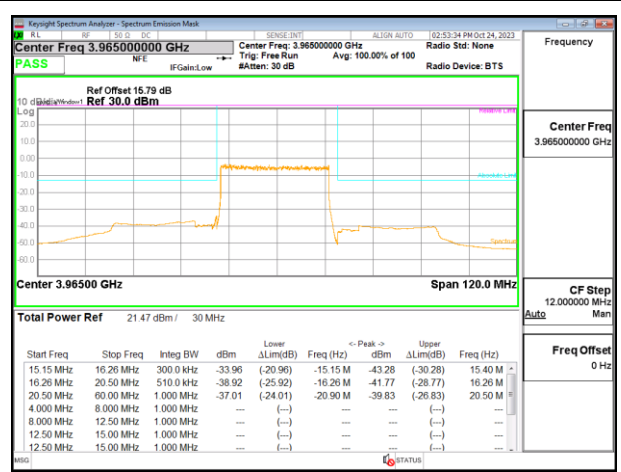
5G NR n77 30MHz QPSK High Channel RB75-0
