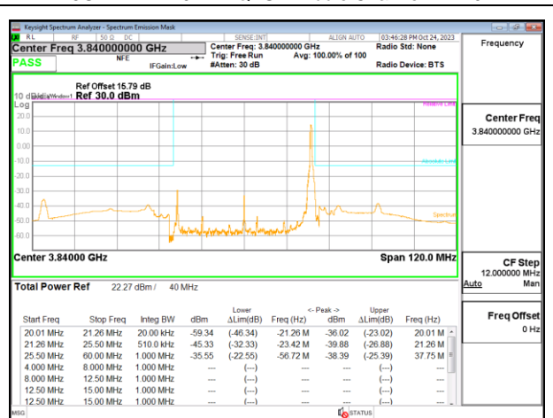
5G NR n77 40MHz QPSK Middle Channel RB1-105
