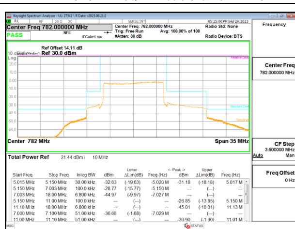
LTE B13 10MHz 16QAM Middle Channel RB50-0
