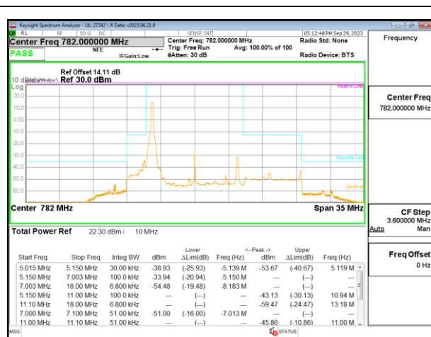
LTE B13 10MHz 16QAM Middle Channel RB1-0
