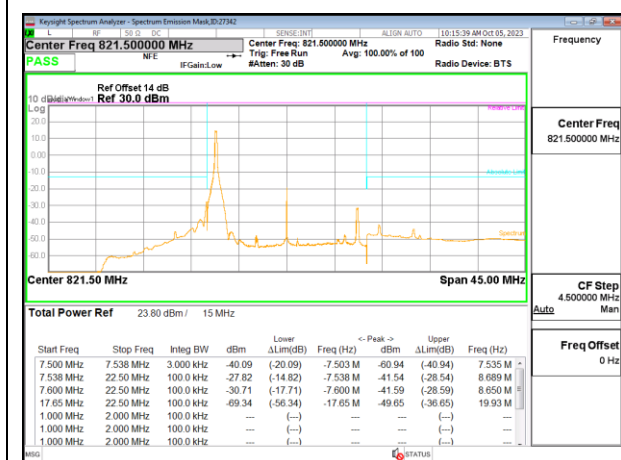
LTE B26 15MHz QPSK Middle Channel RB1-0
