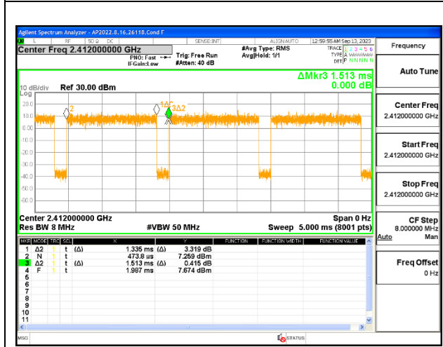
DUTY CYCLE 802.11n 1TX MODE
