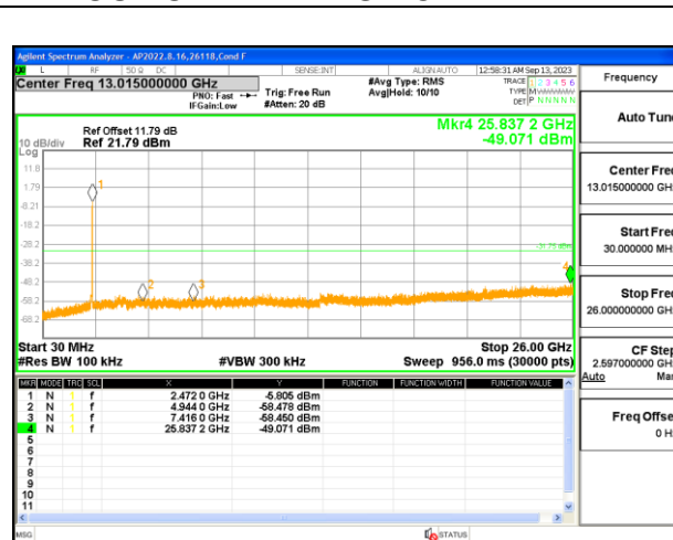
OUT-OF-BAND HIGH CHANNEL 13
