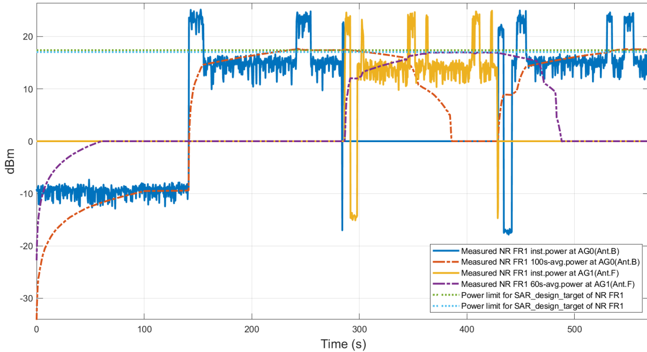
Plot.1 : Conducted Tx power for NR :
