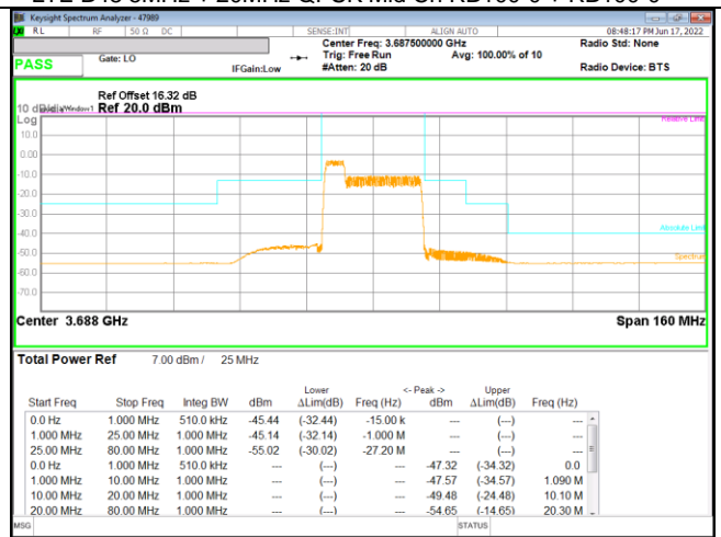
LTE B48 5MHz + 20MHz QPSK High Ch RB100-0 + RB100-0
