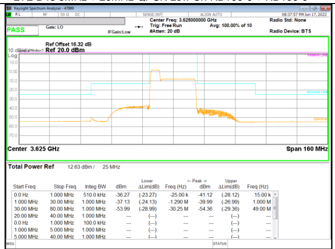
LTE B48 5MHz + 20MHz QPSK Mid Ch RB100-0 + RB100-0
