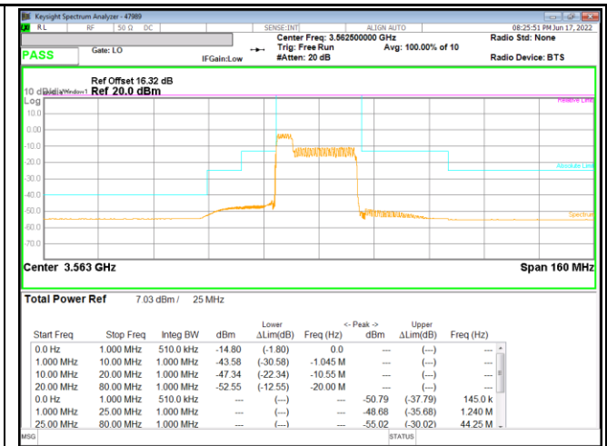
LTE B48 5MHz + 20MHz 16QAM Low Ch RB100-0 + RB100-0
