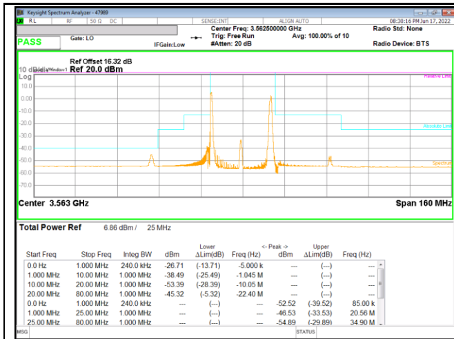
LTE B48 5MHz + 20MHz 16QAM Low Ch RB1-0 + RB1-99
