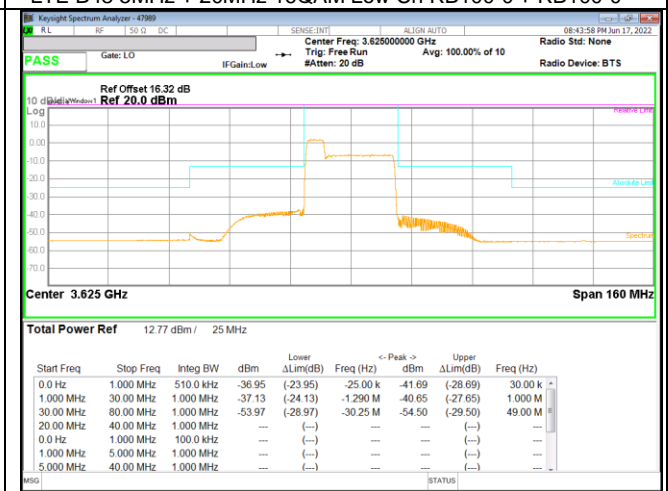
LTE B48 5MHz + 20MHz 16QAM Mid Ch RB100-0 + RB100-0
