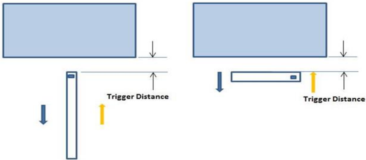
Proximity Sensor Trigger Distance Assessment KDB 616217 §6.2, Edge 3 , Edge 4
