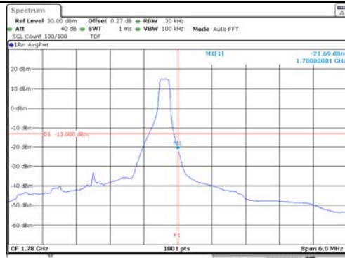
3M BW 16QAM High ch. FRB
