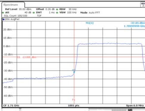
3M BW 16QAM Low ch. 1RB
