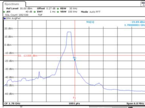
3M BW QPSK High ch. FRB
