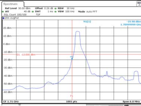
3M BW QPSK Low ch. FRB
