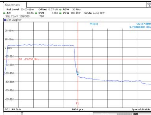
3M BW 16QAM High ch. 1RB
