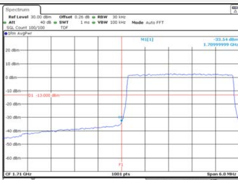
3M BW 16QAM Low ch. FRB
