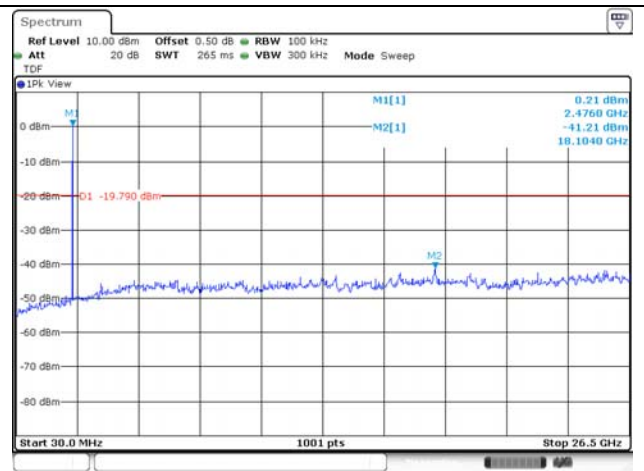
Conducted spurious / 2 472 MHz
