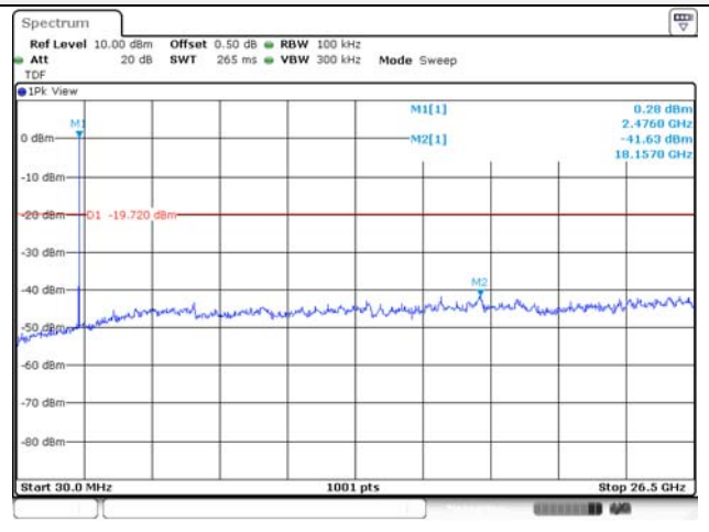
Conducted spurious / 2 472 MHz
