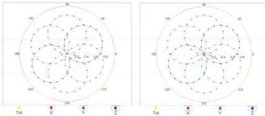
f=600 MHz,TEM
