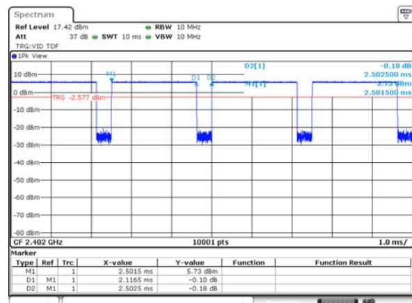
1M Bits/s, 255 Packet
