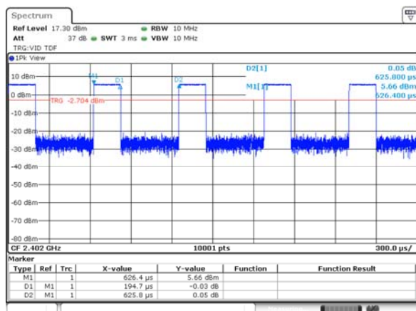
2M Bits/s, 37 Packet
