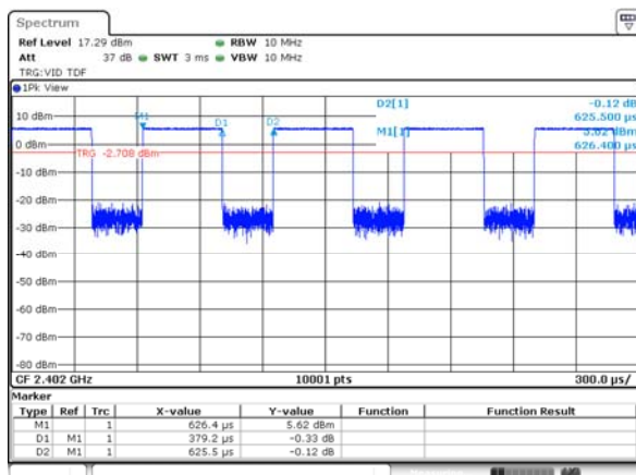
1M Bits/s, 37 Packet
