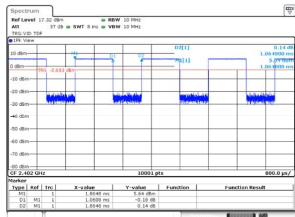
2M Bits/s, 255 Packet
