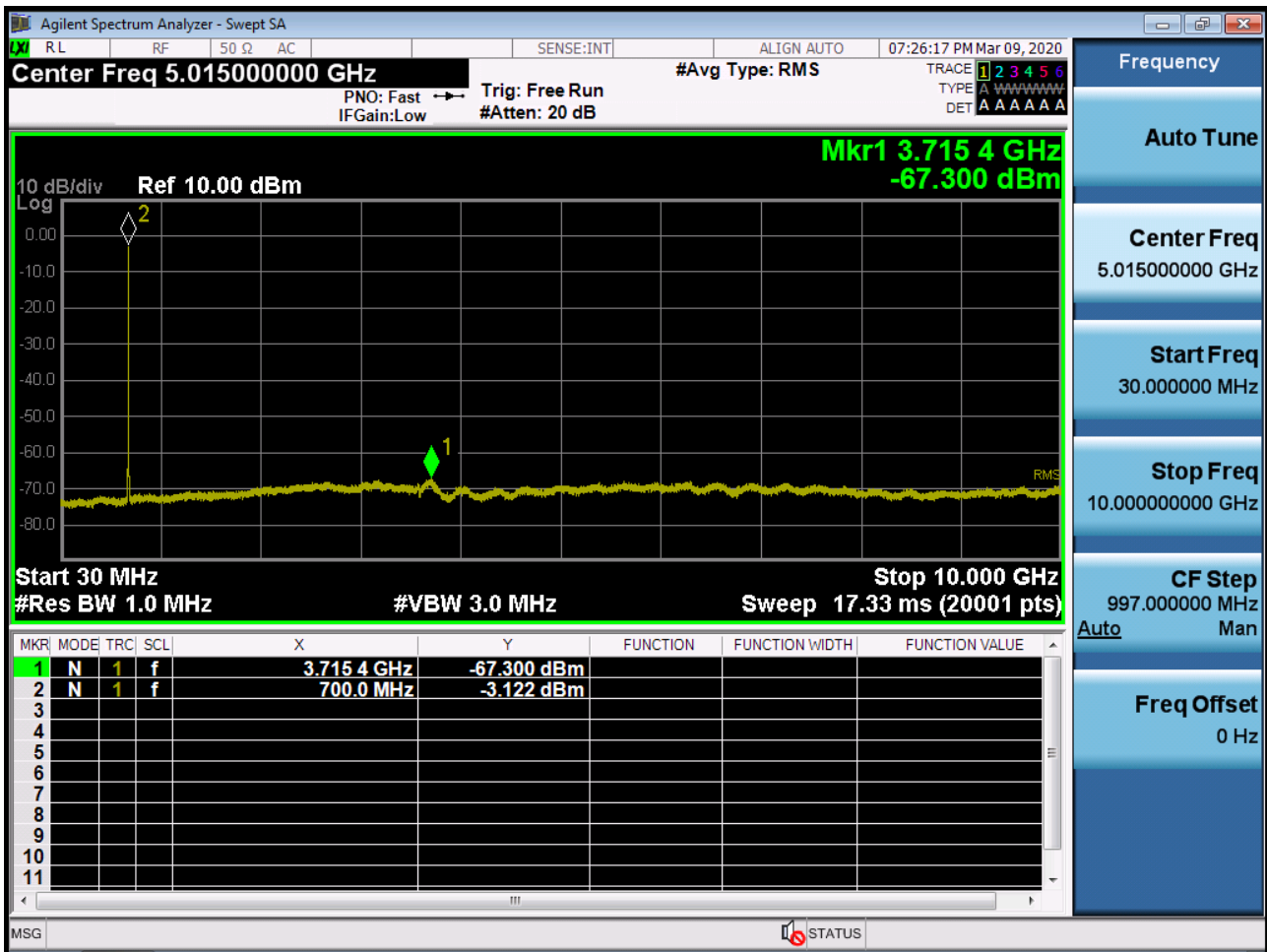
BAND 12. Conducted Spurious Plot _ (23017ch_1.4MHz_QPSK_RB 1_0)
