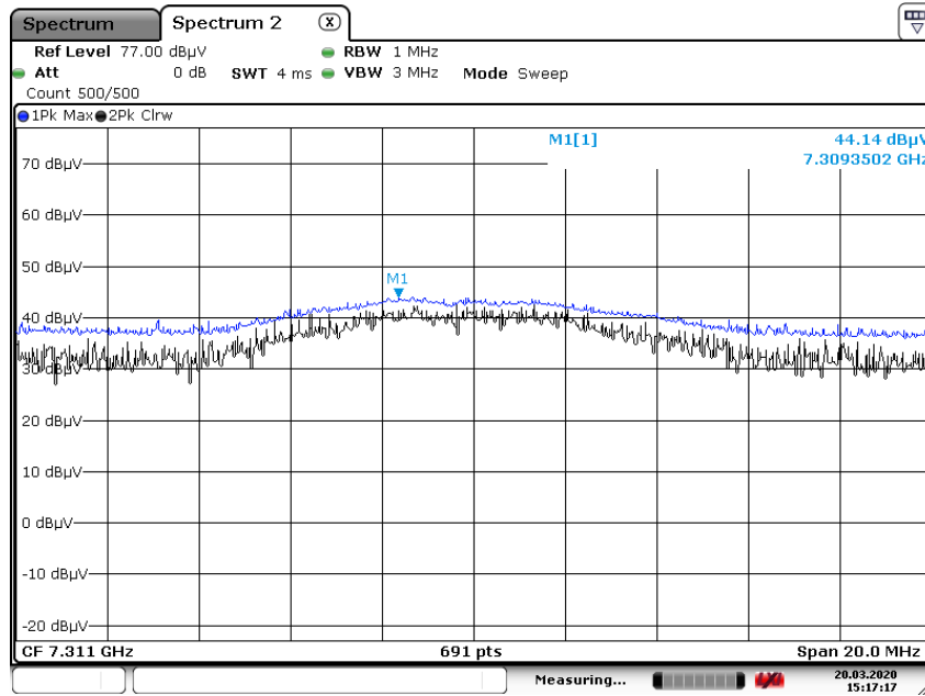
Radiated Spurious Emissions plot – Peak Reading (802.11b_1 Mbps, Ch.6 3rd Harmonic)
