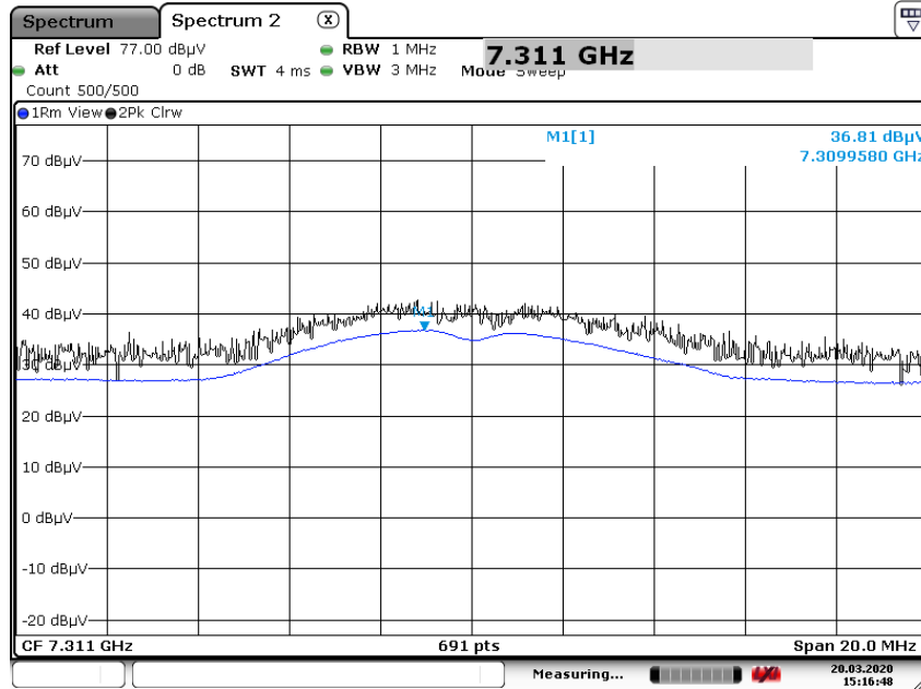
Radiated Spurious Emissions plot – Average Reading (802.11b_1 Mbps, Ch.6 3rd Harmonic)
