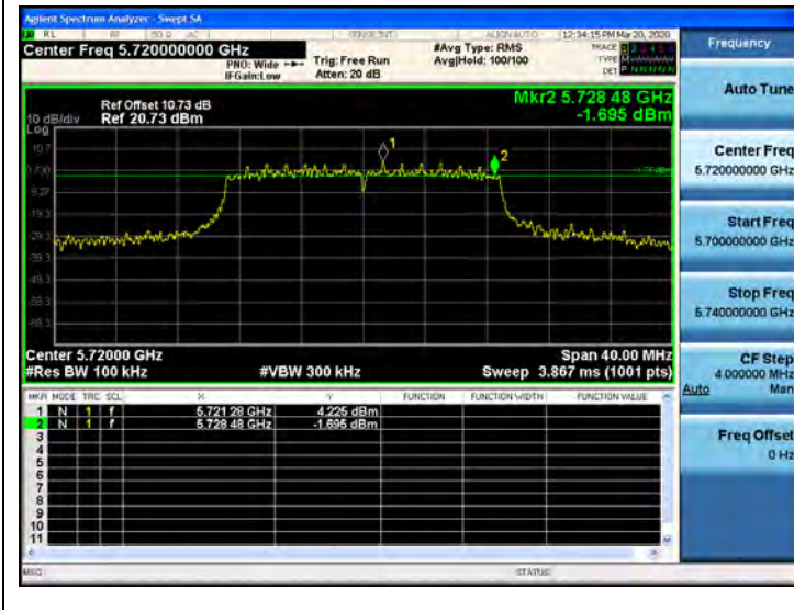
802.11ac_VHT20 CH.144
