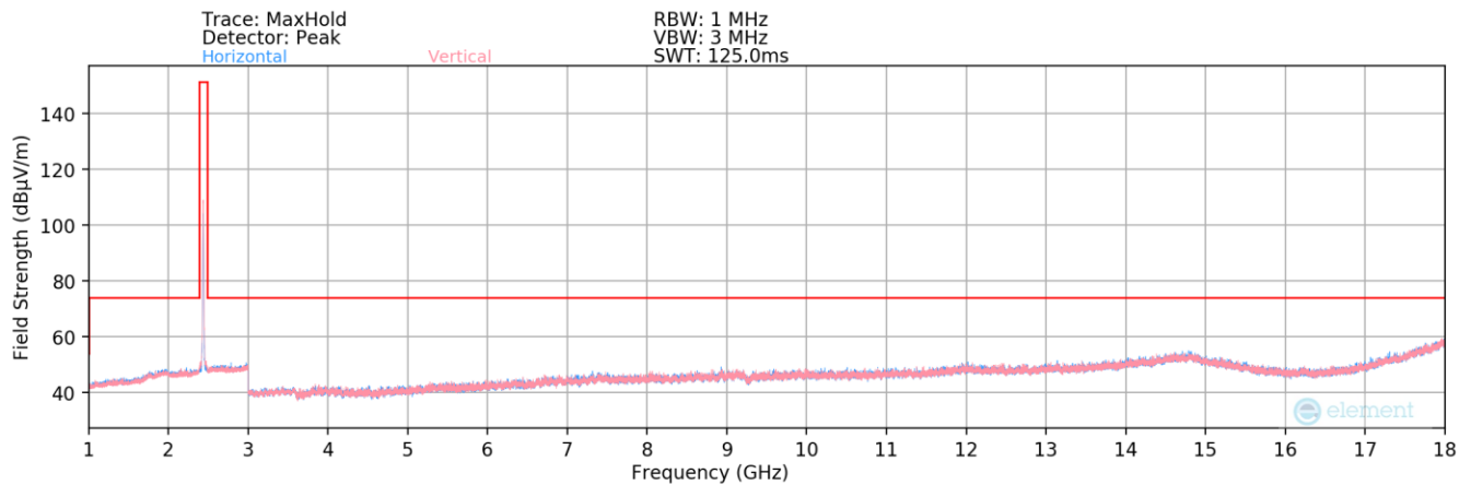
Plot 7-38. Radiated Spurious Plot above 1GHz (802.11b – Ch. 1)
