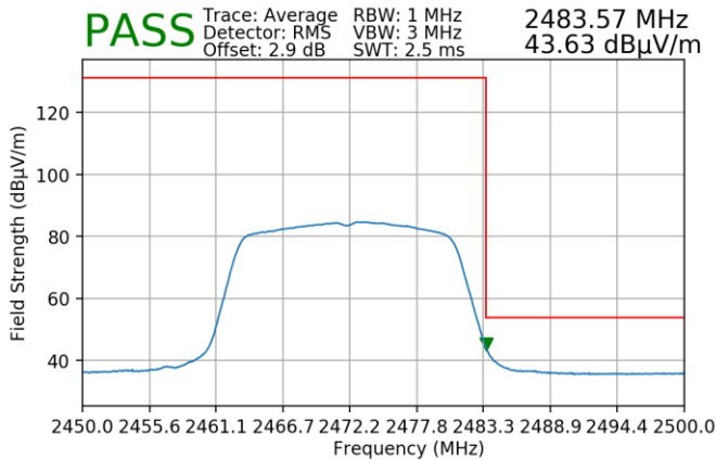
Plot 7-48. Radiated Restricted Upper Band Edge Measurement (Average)
