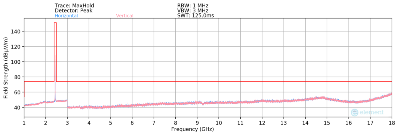
Plot 7-39. Radiated Spurious Plot above 1GHz (802.11b – Ch. 6)
