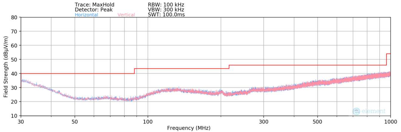
Plot 7-37. Radiated Spurious Plot below 1GHz
