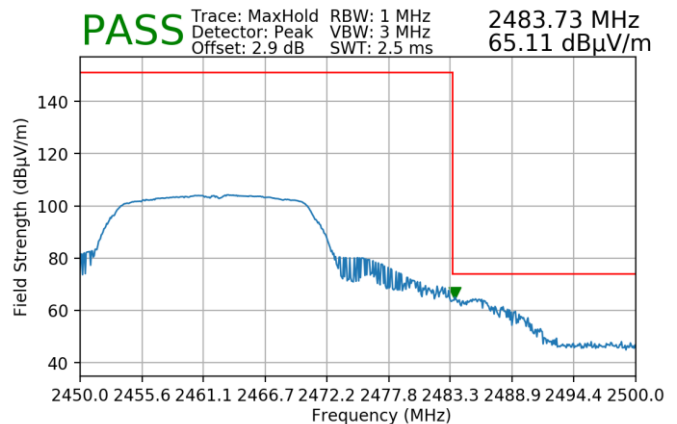
Plot 7-45. Radiated Restricted Upper Band Edge Measurement (Peak)
