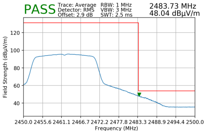
Plot 7-44. Radiated Restricted Upper Band Edge Measurement (Average)
