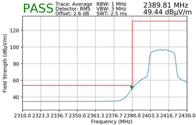
Plot 7-42. Radiated Restricted Lower Band Edge Measurement (Average)
