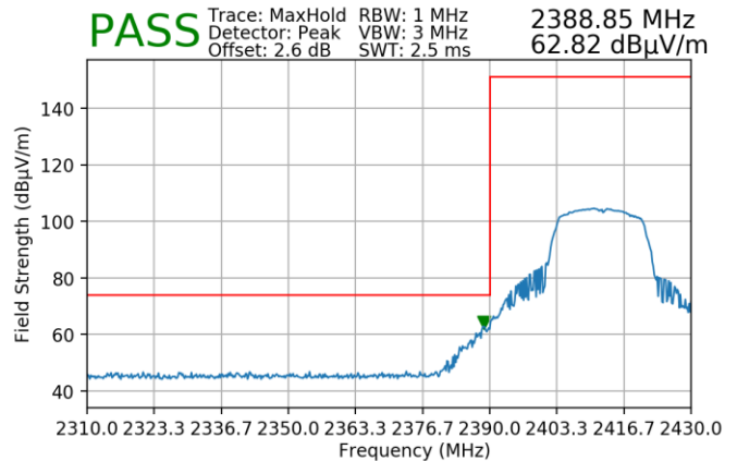
Plot 7-43. Radiated Restricted Lower Band Edge Measurement (Peak)
