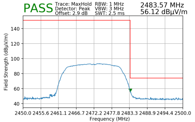
Plot 7-49. Radiated Restricted Upper Band Edge Measurement (Peak)
