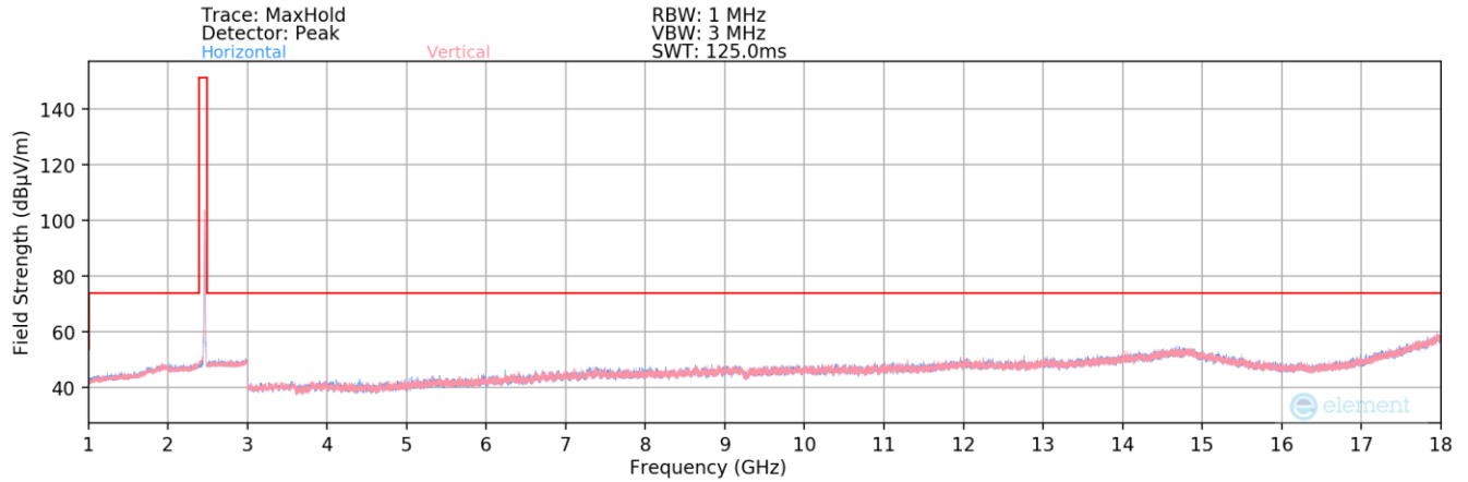
Plot 7-40. Radiated Spurious Plot above 1GHz (802.11b – Ch. 11)
