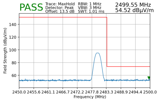
Plot 7-30. Radiated Restricted Upper Band Edge Measurement (Peak)
