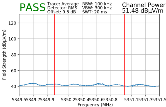
Plot 7-53. Radiated Upper Band Edge Plot (Average – UNII Band 2A)
