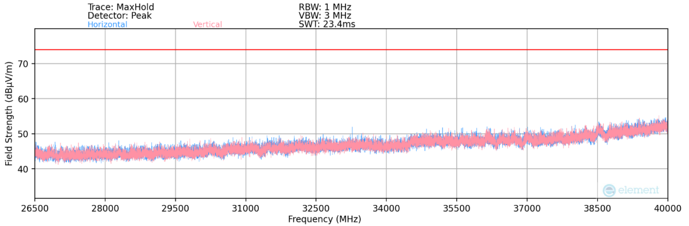
Plot 7-39. Radiated Spurious Plot 26.5GHz – 40GHz (802.11a)
