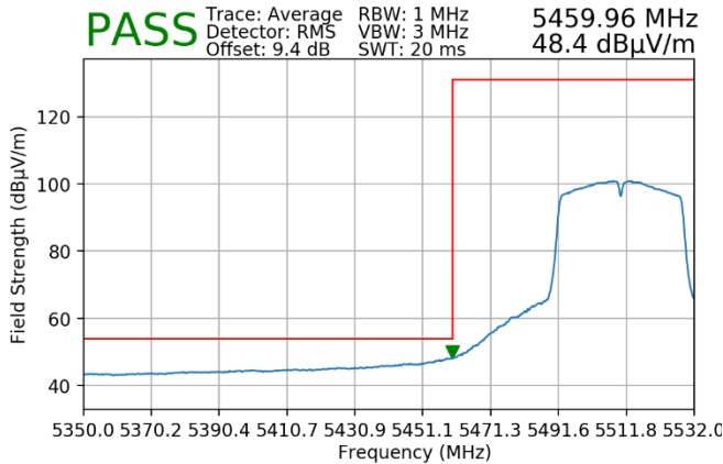
Plot 7-55. Radiated Lower Band Edge Plot (Average – UNII Band 2C)
