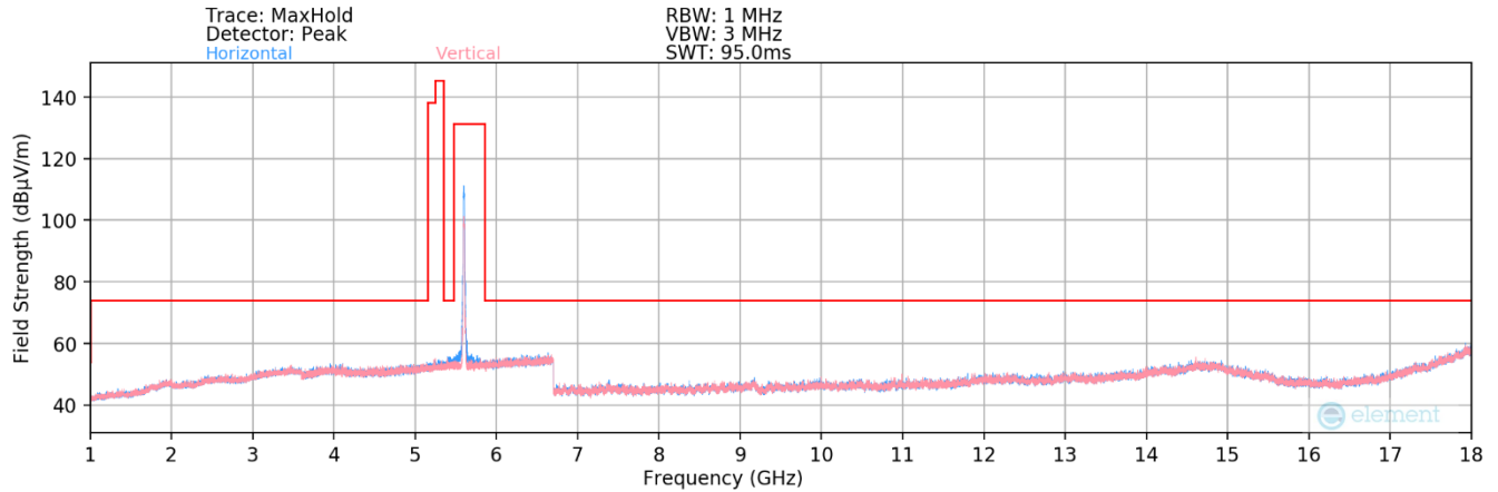
Plot 7-36. Radiated Spurious Plot above 1GHz (802.11a – UNII Band 2C Ch. 120)
