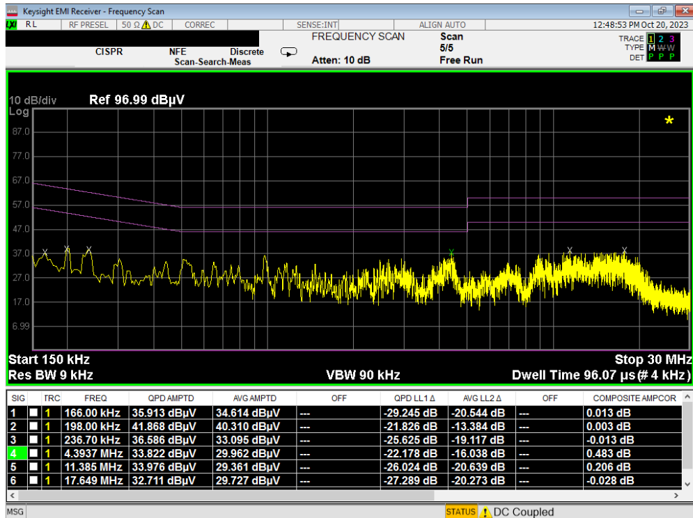
Plot 7-68. Line Conducted Plot with 802.11a UNII Band 2A (N)
