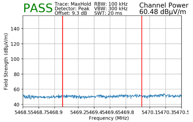
Plot 7-49. Radiated Lower Band Edge Plot (Peak – UNII Band 2C)
