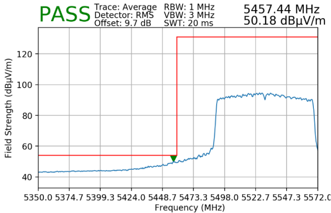
Plot 7-62. Radiated Lower Band Edge Plot (Average – UNII Band 2C)
