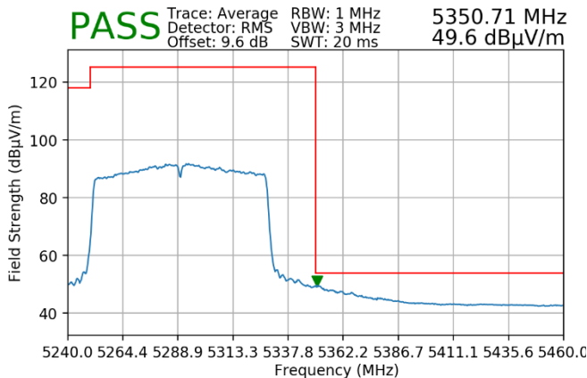
Plot 7-60. Radiated Upper Band Edge Plot (Average – UNII Band 2A)
