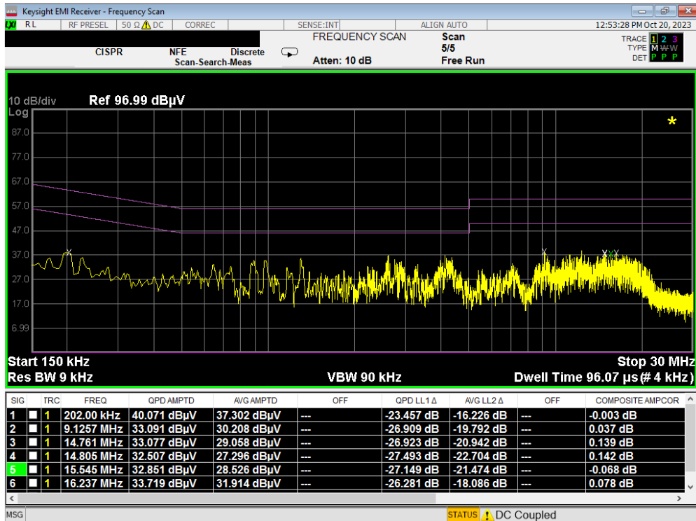
Plot 7-70. Line Conducted Plot with 802.11a UNII Band 2C (N)
