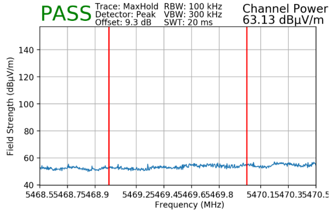
Plot 7-56. Radiated Lower Band Edge Plot (Peak – UNII Band 2C)
