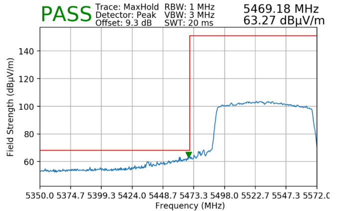
Plot 7-63. Radiated Lower Band Edge Plot (Peak – UNII Band 2C)
