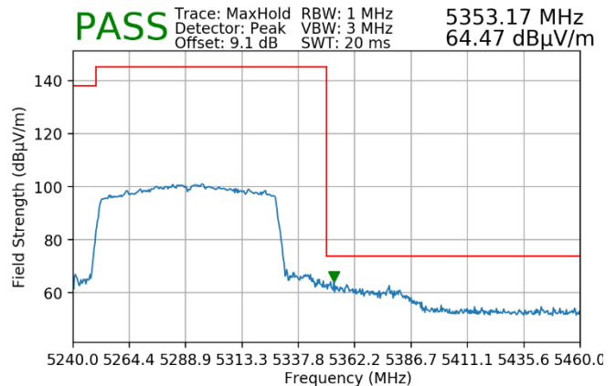
Plot 7-61. Radiated Upper Band Edge Plot (Peak – UNII Band 2A)
