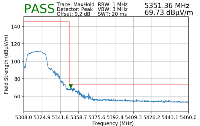
Plot 7-47. Radiated Upper Band Edge Plot M (Peak – UNII Band 2A)
