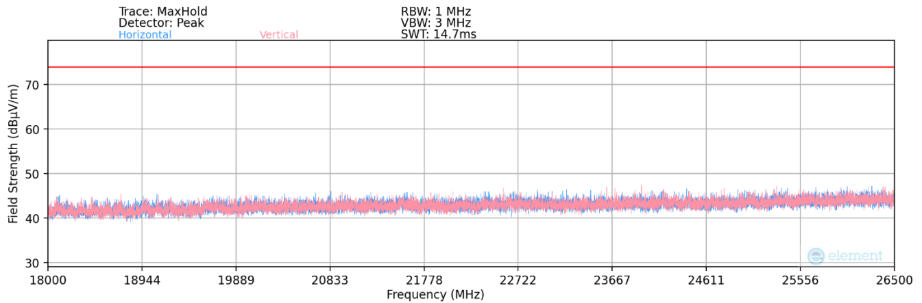
Plot 7-38. Radiated Spurious Plot 18GHz – 26.5GHz (802.11a)
