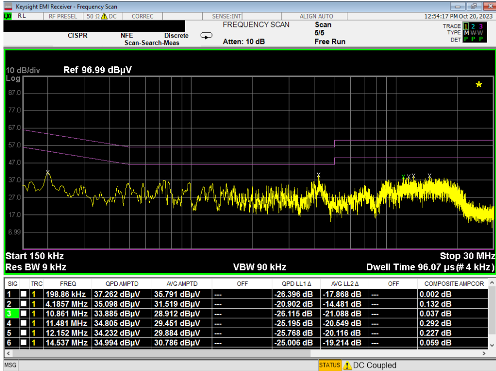
Plot 7-69. Line Conducted Plot with 802.11a UNII Band 2C (L1)
