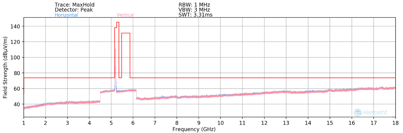
Plot 7-34. Radiated Spurious Plot above 1GHz (802.11a – UNII Band 1 Ch. 40)
