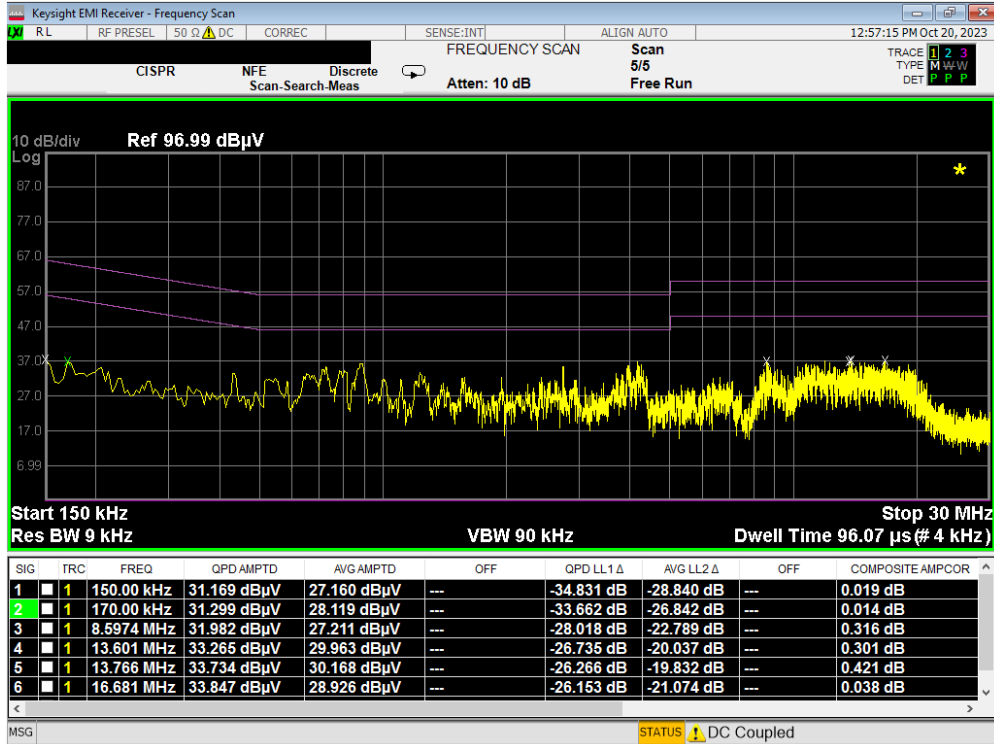
Plot 7-71. Line Conducted Plot with 802.11a UNII Band 3 (L1)
