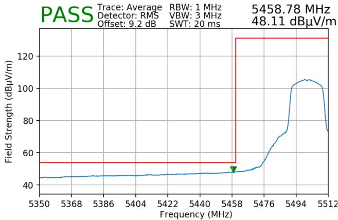
Plot 7-48. Radiated Lower Band Edge Plot (Average – UNII Band 2C)
