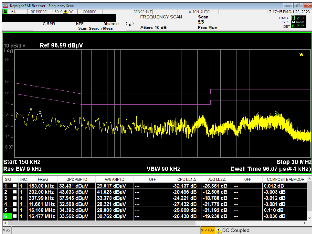
Plot 7-66. Line Conducted Plot with 802.11a UNII Band 1 (N)
