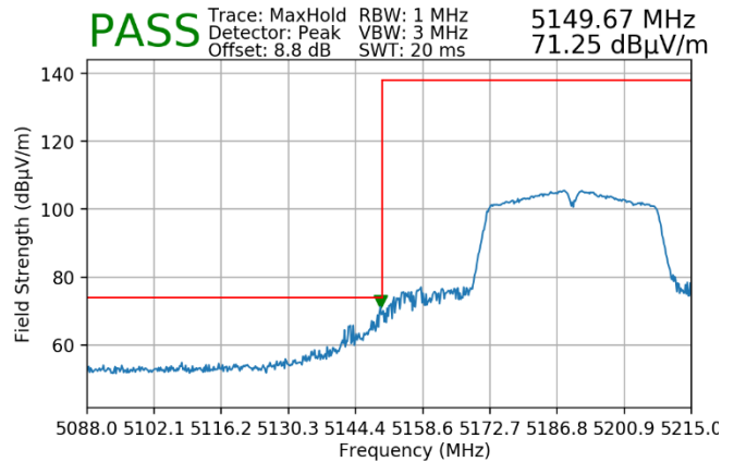
Plot 7-52. Radiated Lower Band Edge Plot (Peak – UNII Band 1)
