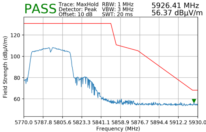
Plot 7-57. Radiated Upper Band Edge Plot (Peak – UNII Band 3)
