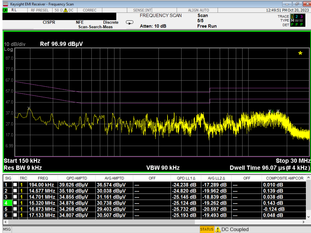
Plot 7-67. Line Conducted Plot with 802.11a UNII Band 2A (L1)
