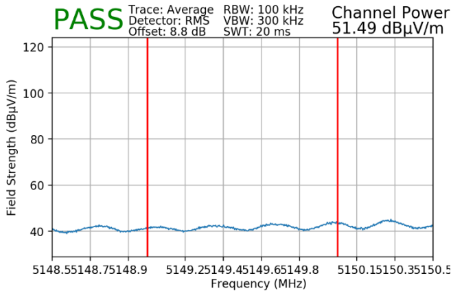
Plot 7-51. Radiated Lower Band Edge Plot (Average – UNII Band 1)
