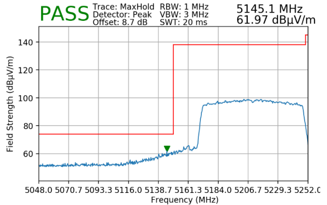
Plot 7-59. Radiated Lower Band Edge Plot (Peak – UNII Band 1)
