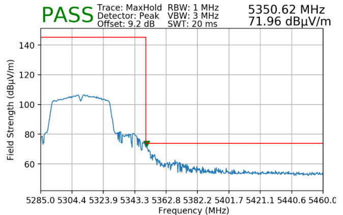
Plot 7-54. Radiated Upper Band Edge Plot (Peak – UNII Band 2A)
