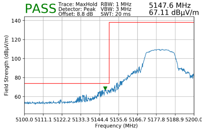
Plot 7-45. Radiated Lower Band Edge Plot (Peak – UNII Band 1)
