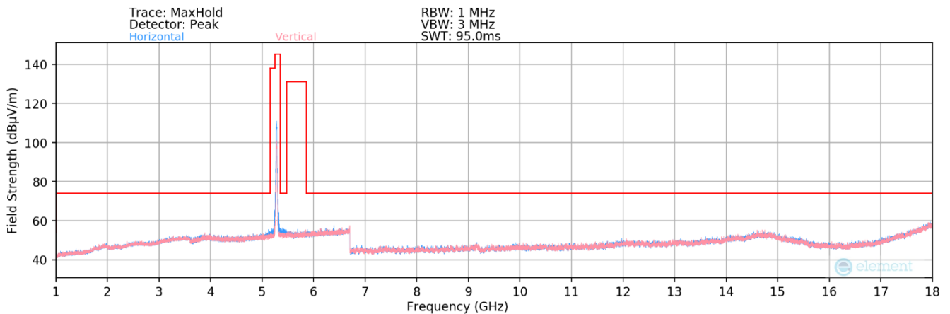
Plot 7-35. Radiated Spurious Plot above 1GHz (802.11a – UNII Band 2A Ch. 56)
