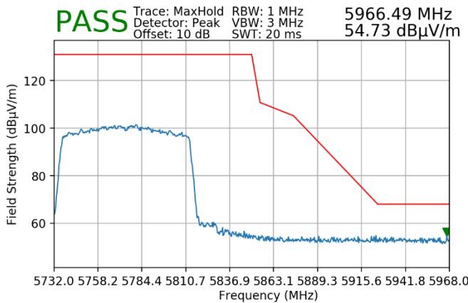
Plot 7-64. Radiated Upper Band Edge Plot (Peak – UNII Band 3)
