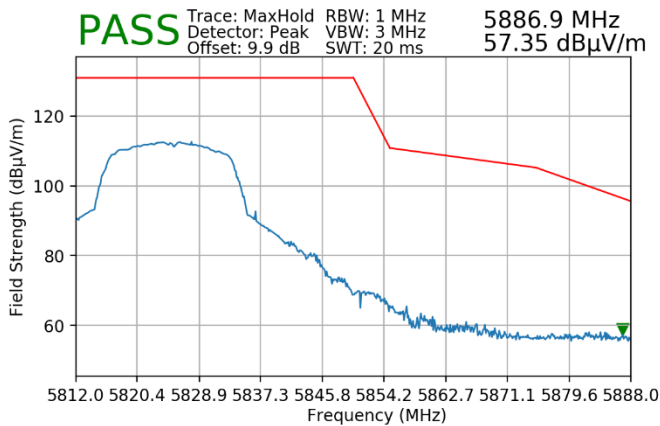
Plot 7-50. Radiated Upper Band Edge Plot (Peak – UNII Band 3)
