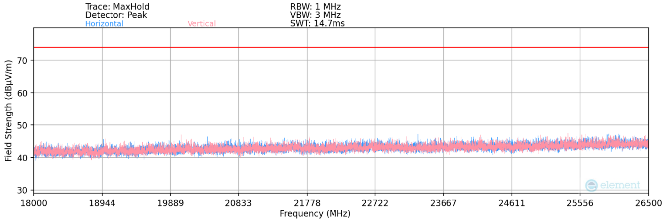
Plot 7-42. Radiated Spurious Plot 18GHz – 26.5GHz (2.4GHz – 5GHz)
