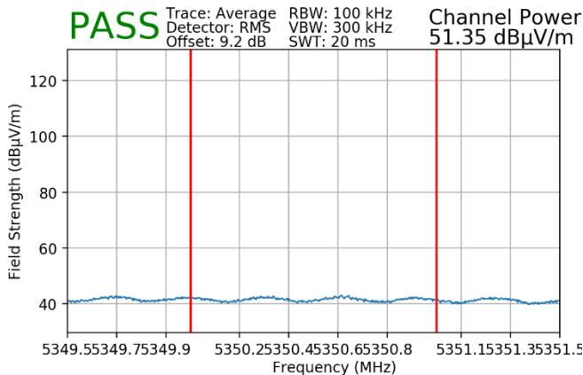
Plot 7-46. Radiated Upper Band Edge Plot (Average – UNII Band 2A)
