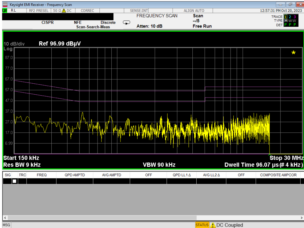
Plot 7-72. Line Conducted Plot with 802.11a UNII Band 3 (N)
