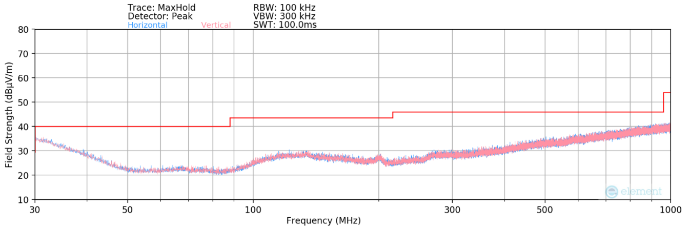
Plot 7-33. Radiated Spurious Plot below 1GHz (802.11a)
