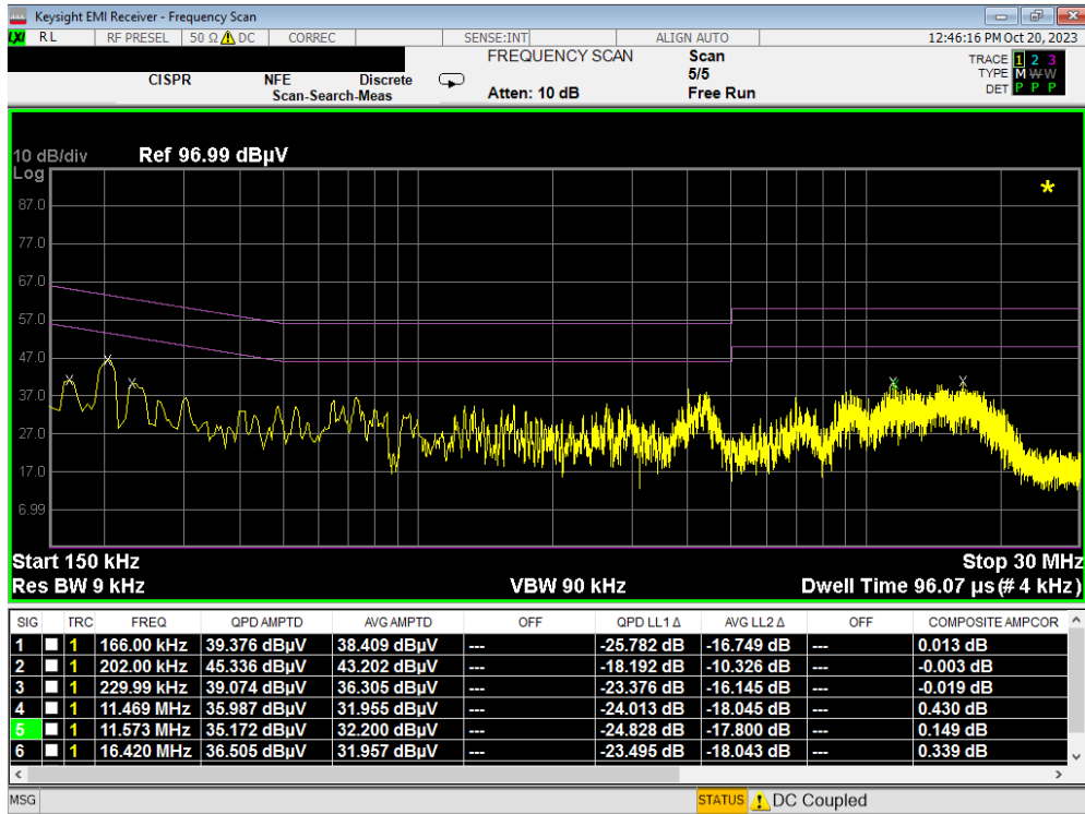
Plot 7-65. Line Conducted Plot with 802.11a UNII Band 1 (L1)
