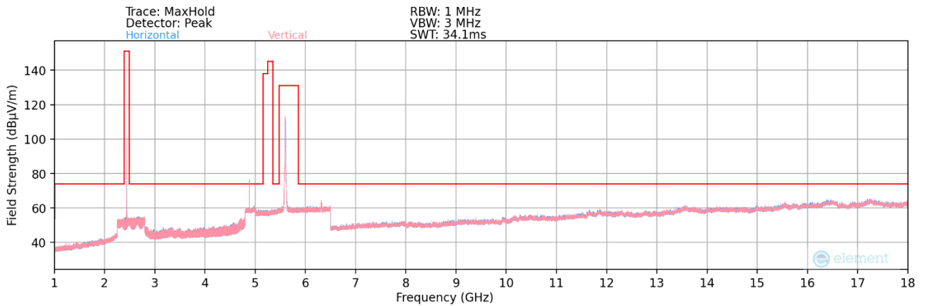
Plot 7-41. Radiated Spurious Plot above 1GHz (2.4GHz – 5GHz)
