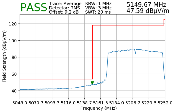
Plot 7-58. Radiated Lower Band Edge Plot (Average – UNII Band 1)
