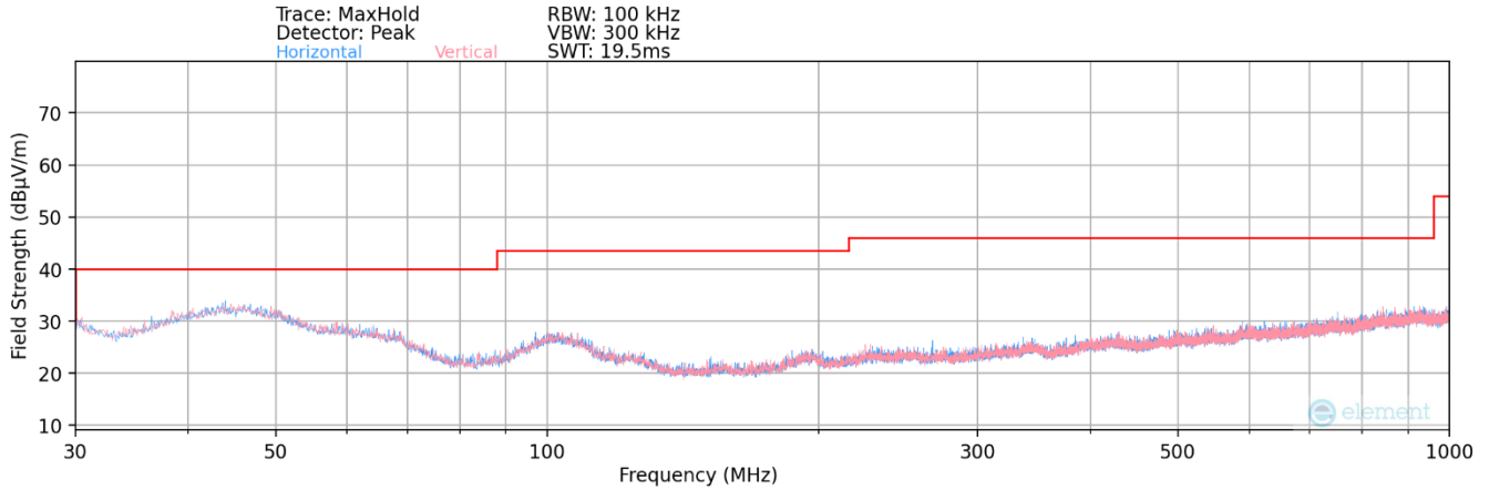
Plot 7-40. Radiated Spurious Plot below 1GHz (2.4GHz – 5GHz)
