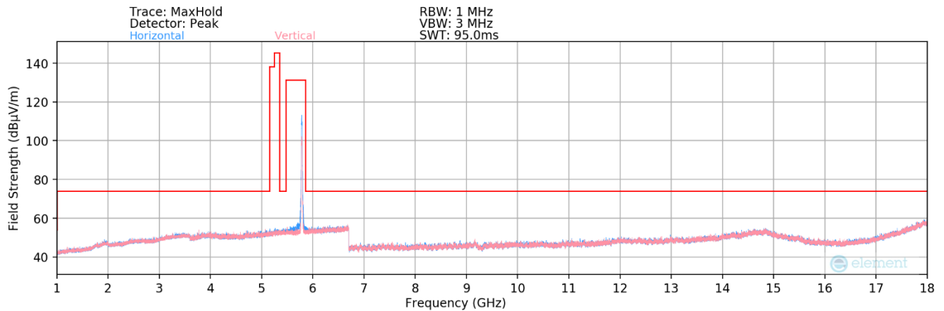
Plot 7-37. Radiated Spurious Plot above 1GHz (802.11a – UNII Band 3 Ch. 157)
