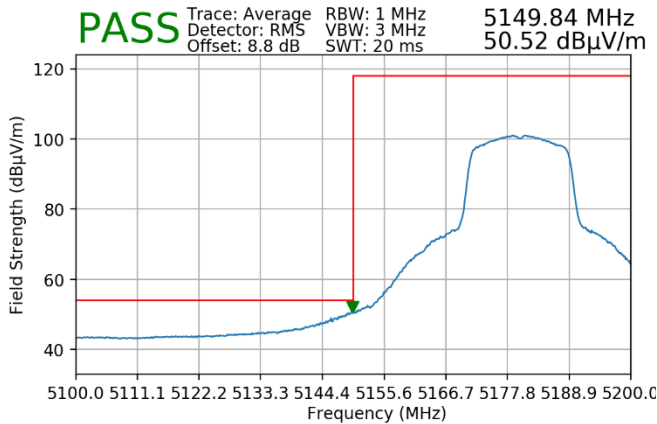
Plot 7-44. Radiated Lower Band Edge Plot (Average – UNII Band 1)
