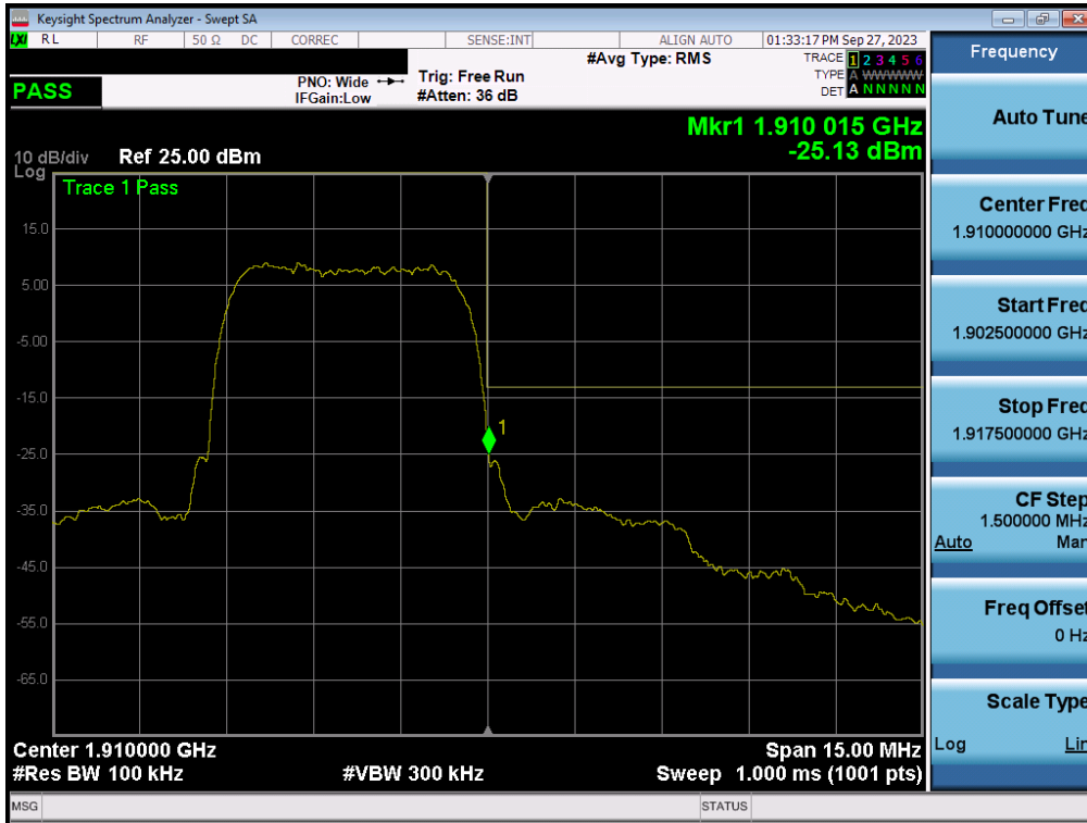
Plot 7-52. Upper Band Edge Plot (WCDMA PCS – Ch. 9538 - Ant1)
