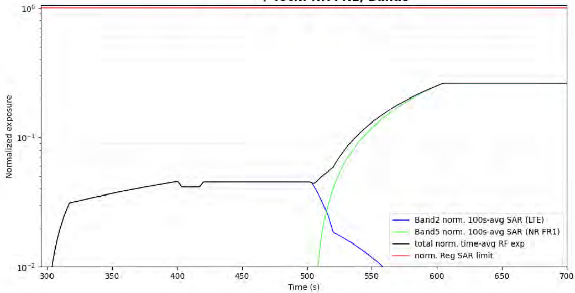
Figure 5- 45 Normalized time-averaged SAR for case 16 (LTE B2, sub6 NR B5)
