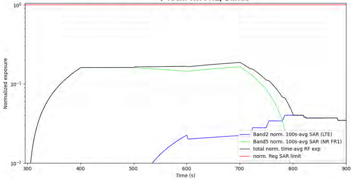
Figure 5- 55 Normalized time-averaged SAR for case 18 (LTE B2, sub6 NR n5)
