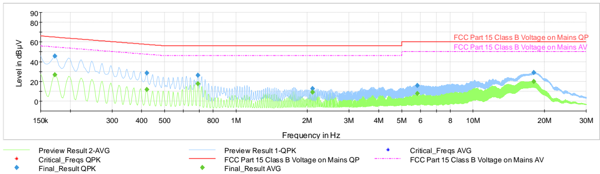
Plot 7-49. Line-Conducted Test Plot (N)
