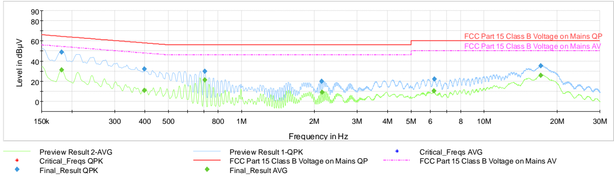
Plot 7-48. Line-Conducted Test Plot (L1)
