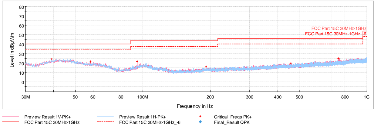
Plot 7-47. Radiated Spurious Plot below 1GHz
