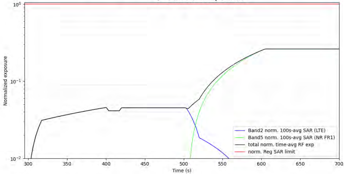
Figure 5- 45 Normalized time-averaged SAR for case 16 (LTE B2, sub6 NR B5)
