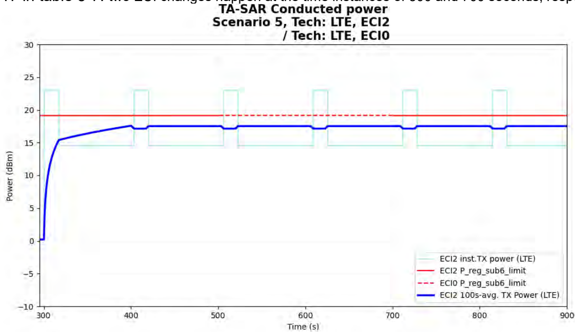
Figure 5- 46 Time-averaged conducted TX power over time for case 17 (LTE B2)
