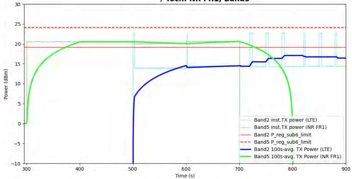
Figure 5- 54 Time-averaged conducted TX power over time for case 18 (LTE B2, sub6 NR n5)
