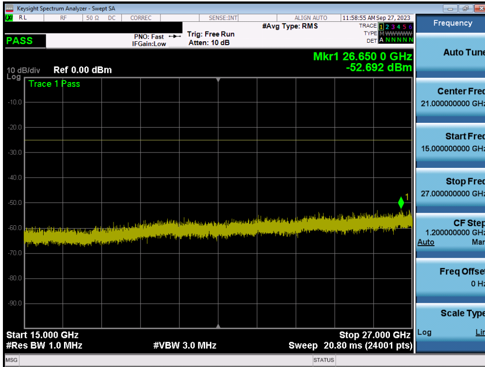
Plot 7-13. Conducted Spurious Plot (LTE Band 41(PC3) - 20MHz QPSK - RB Size 1, RB Offset 0 - High Channel)
