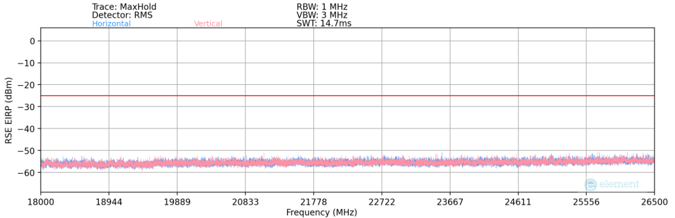
Plot 7-19. Radiated Spurious Plot (LTE Band 41(PC3) – Above 18GHz)
