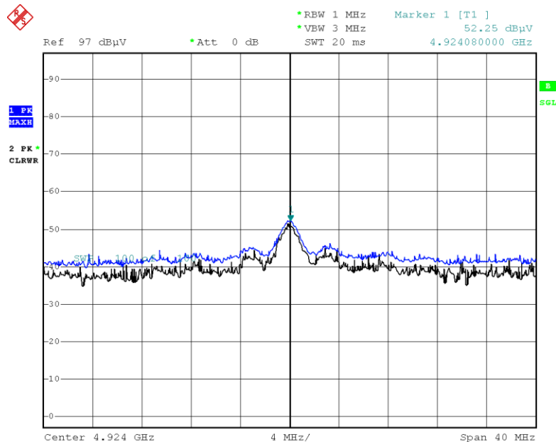
Radiated Spurious Emissions plot – Peak Result (802.11b_1 Mbps, Ch.11 2nd Harmonic)
