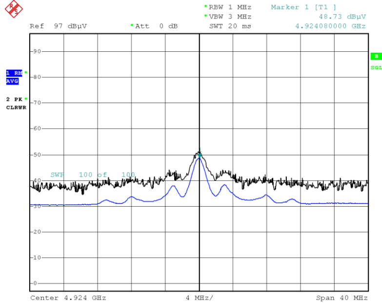
Radiated Spurious Emissions plot – Average Result (802.11b_1 Mbps, Ch.11 2nd Harmonic)
