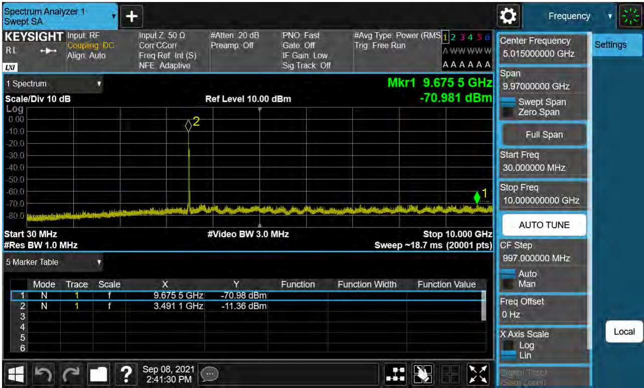
Sub6 n77. Conducted Spurious Plot_1 (633334ch_20 MHz_BPSK)
