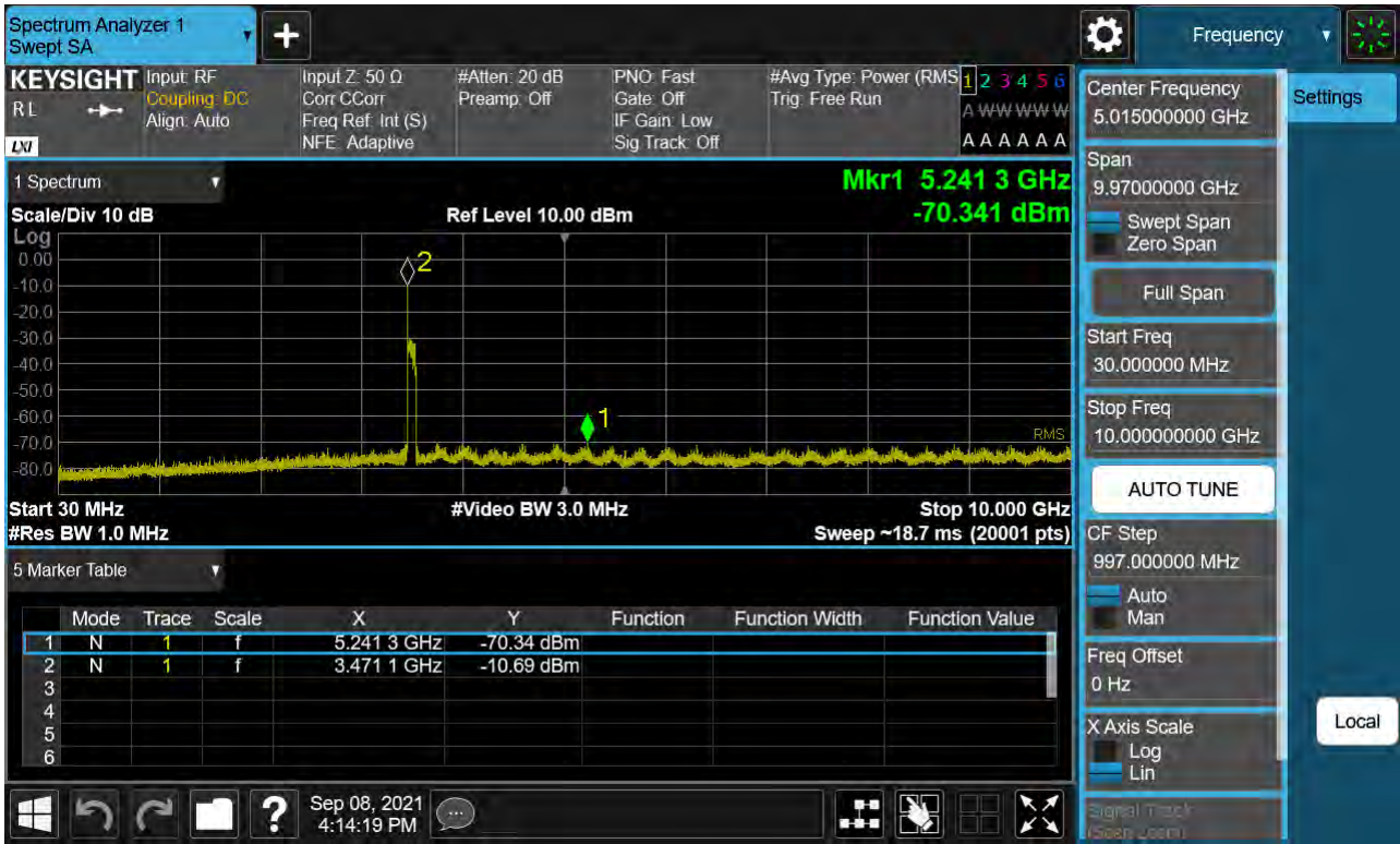
Sub6 n77. Conducted Spurious Plot_1 (634000ch_80 MHz_BPSK)
