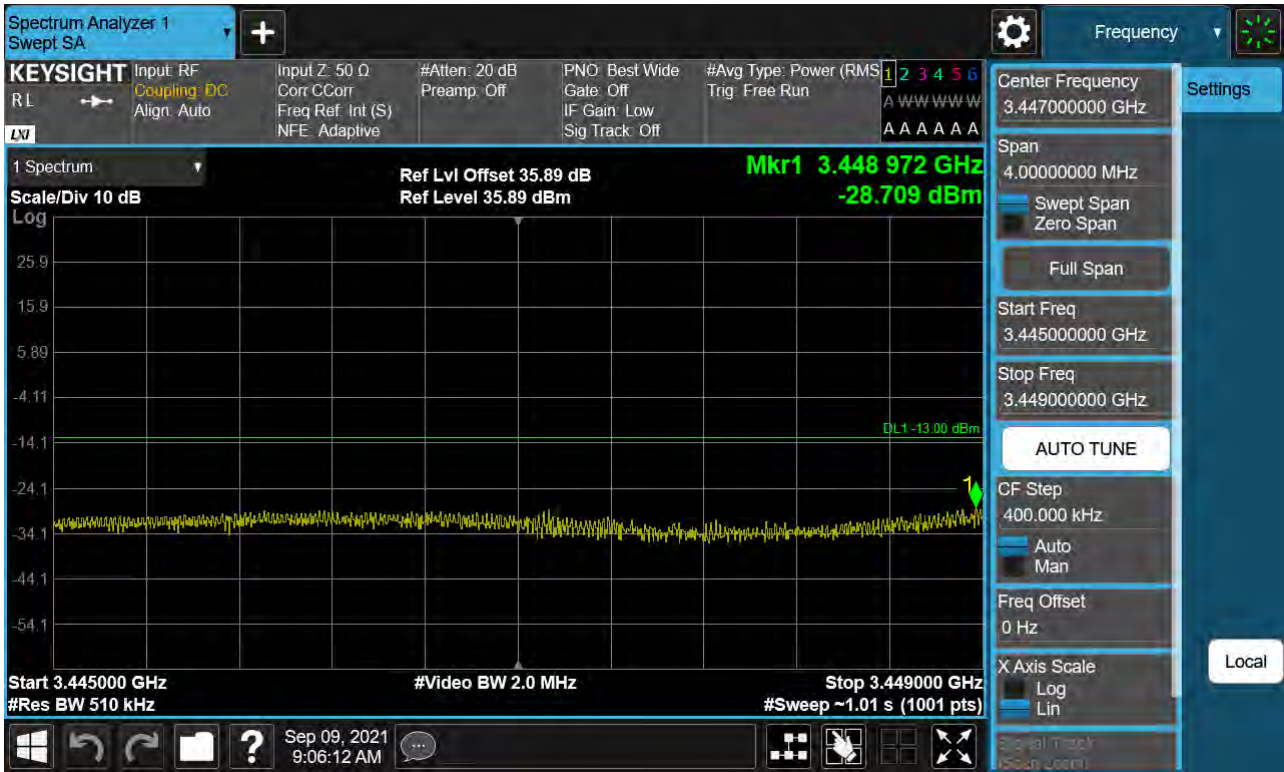
Sub6 n77. Low Band Edge Plot (15 M BW Ch.630500 BPSK 1RB)(2)
