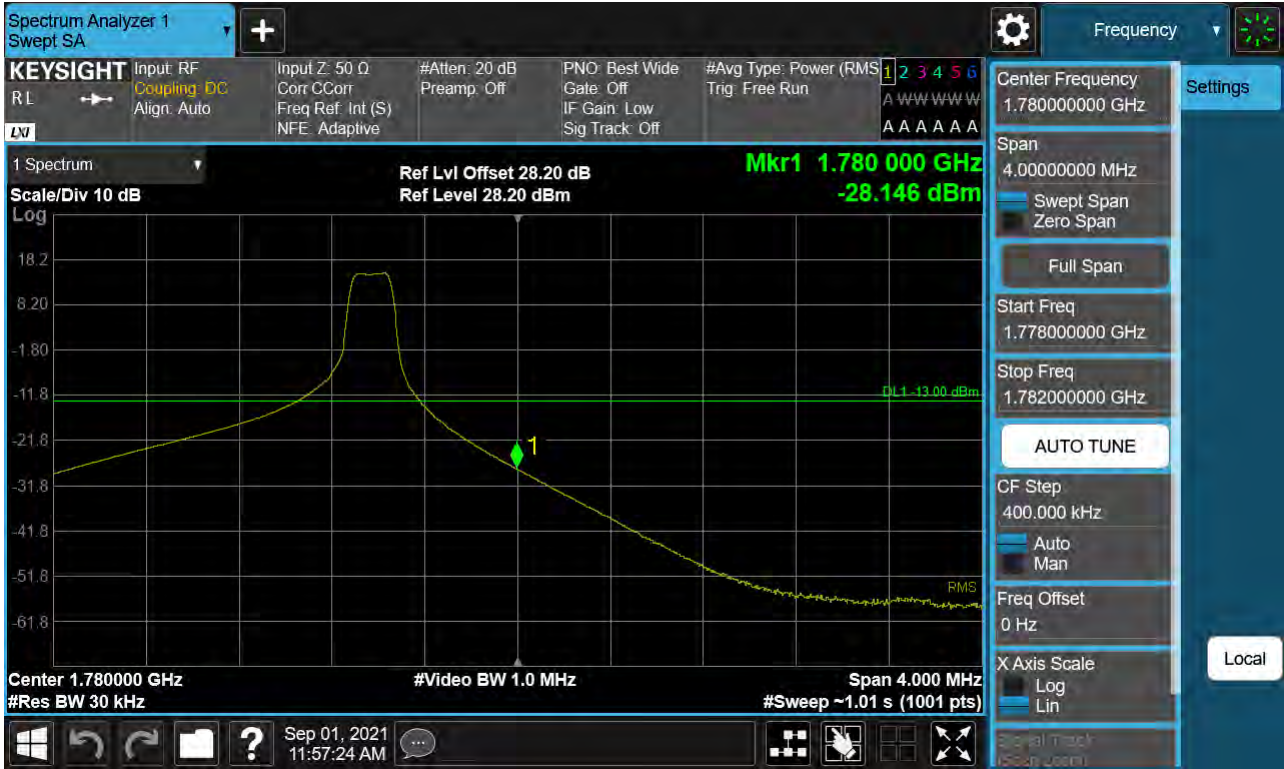
Sub6 n66. Upper Band Edge Plot (25 M BW Ch.353500 BPSK_RB1_Offset 132) -1
