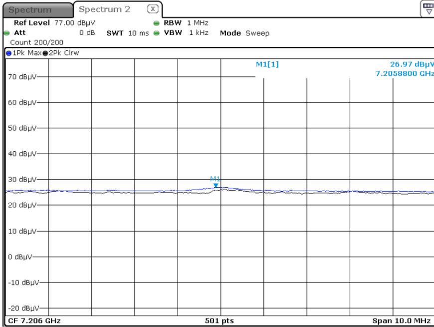
Radiated Spurious Emissions plot – Average Result (GFSK, Ch.0 3rd Harmonic, Y-V)
