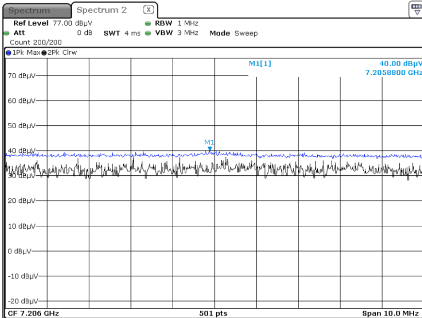
Radiated Spurious Emissions plot – Peak Result ( \pi/4 DQPSK, Ch.0 3rd Harmonic, Y-V)
