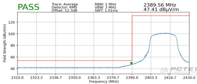
Plot 7-41. Radiated Restricted Lower Band Edge Measurement (Average)
