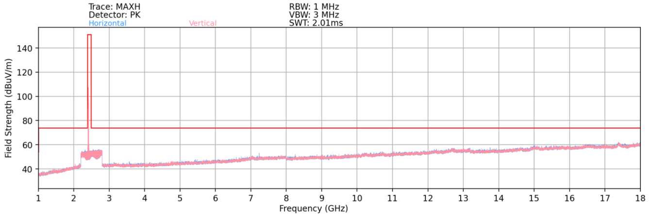
Plot 7-37. Radiated Spurious Plot above 1GHz (802.11b – Ch. 1)
