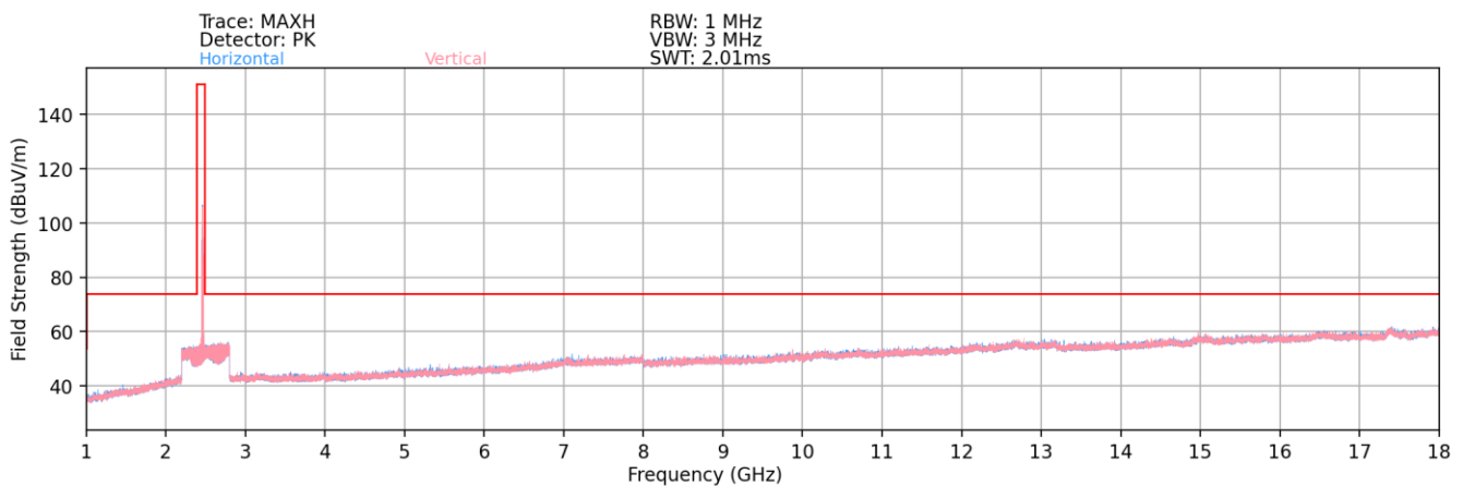
Plot 7-39. Radiated Spurious Plot above 1GHz (802.11b – Ch. 11)
