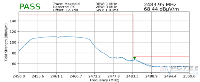
Plot 7-44. Radiated Restricted Upper Band Edge Measurement (Peak)
