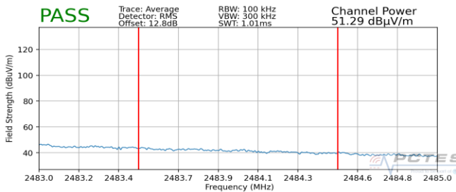
Plot 7-47. Radiated Restricted Upper Band Edge Measurement (Average)
