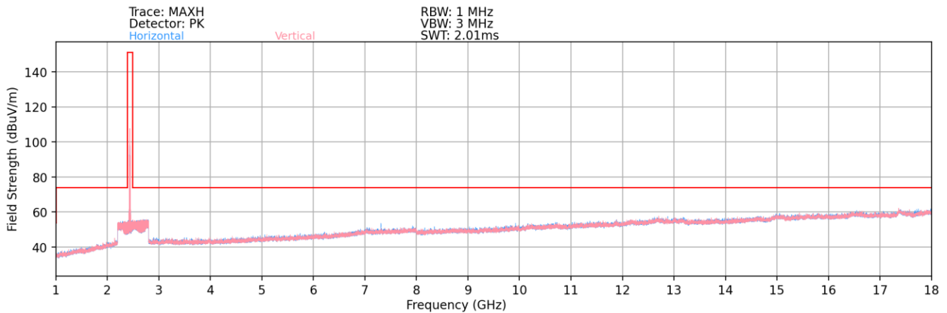
Plot 7-38. Radiated Spurious Plot above 1GHz (802.11b – Ch. 6)
