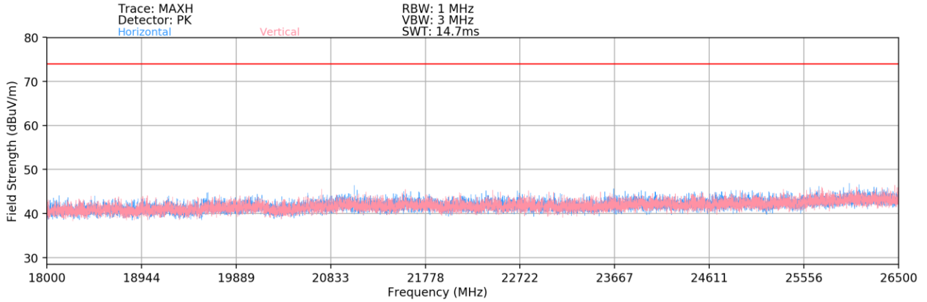
Plot 7-40. Radiated Spurious Plot above 18GHz
