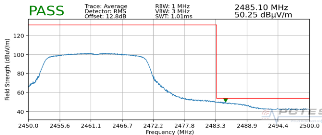
Plot 7-43. Radiated Restricted Upper Band Edge Measurement (Average)
