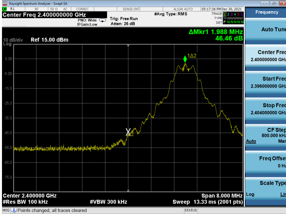
Plot 7-26. Band Edge Plot (Bluetooth (LE), 500kbps – Ch. 0)
