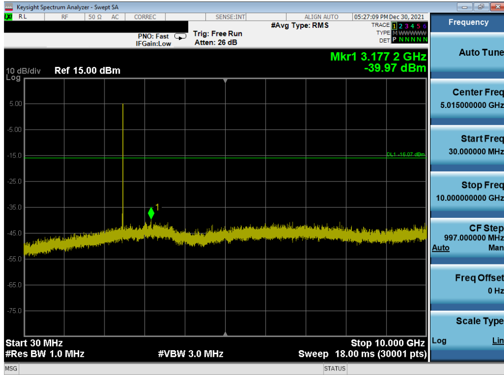
Plot 7-36. Conducted Spurious Plot (Bluetooth (LE), 1Mbps – Ch. 39)
