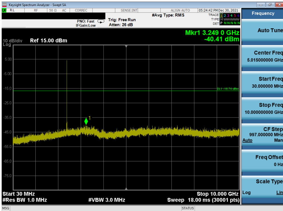
Plot 7-32. Conducted Spurious Plot (Bluetooth (LE), 1Mbps – Ch. 0)
