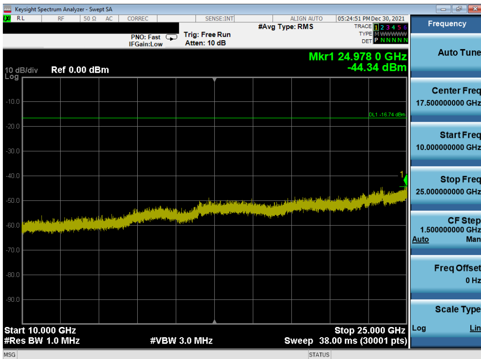
Plot 7-33. Conducted Spurious Plot (Bluetooth (LE), 1Mbps - Ch. 0)
