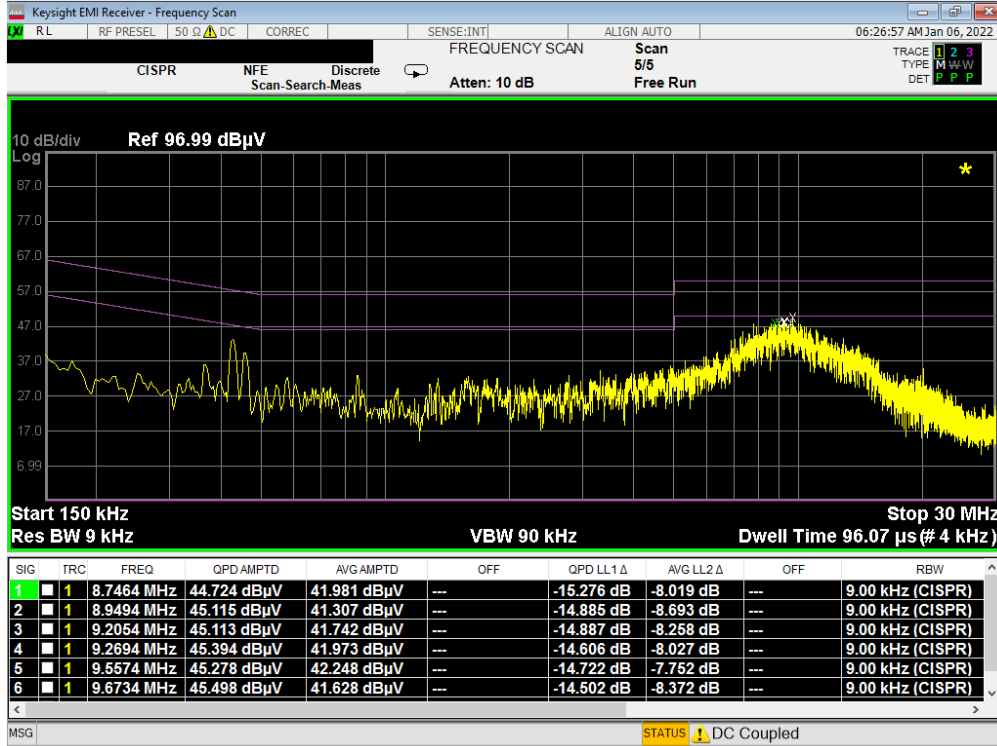
Plot 7-40. Line Conducted Plot with Bluetooth LE (L1)
