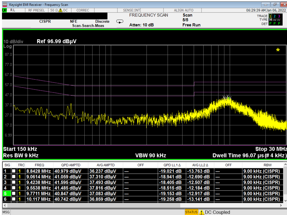
Plot 7-41. Line Conducted Plot with Bluetooth LE (N)
