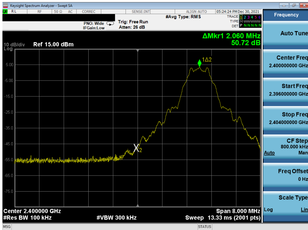
Plot 7-28. Band Edge Plot (Bluetooth (LE), 1Mbps – Ch. 0)
