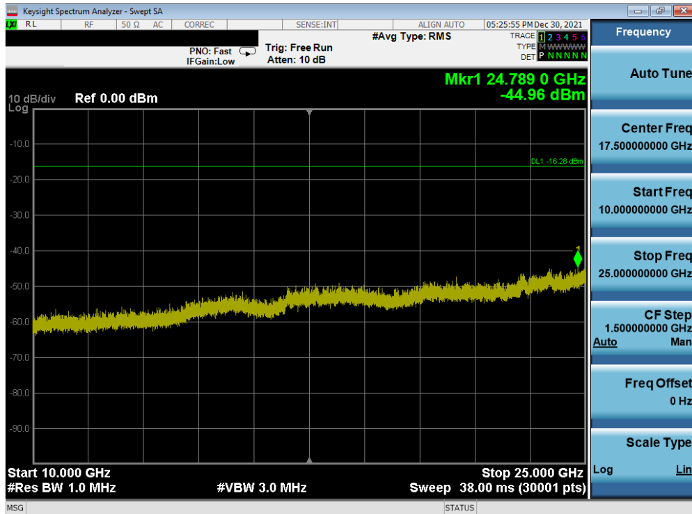
Plot 7-35. Conducted Spurious Plot (Bluetooth (LE), 1Mbps – Ch. 19)
