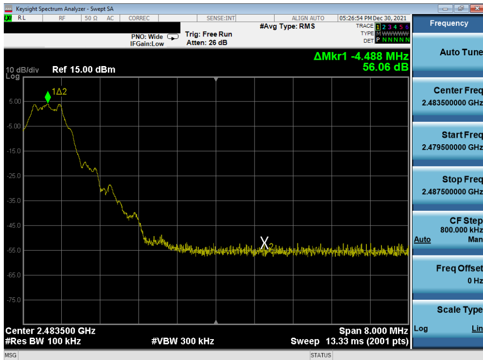
Plot 7-29. Band Edge Plot (Bluetooth (LE), 1Mbps – Ch. 39)
