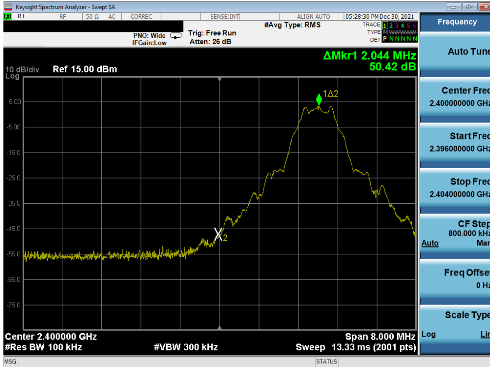
Plot 7-30. Band Edge Plot (Bluetooth (LE), 2Mbps – Ch. 0)
