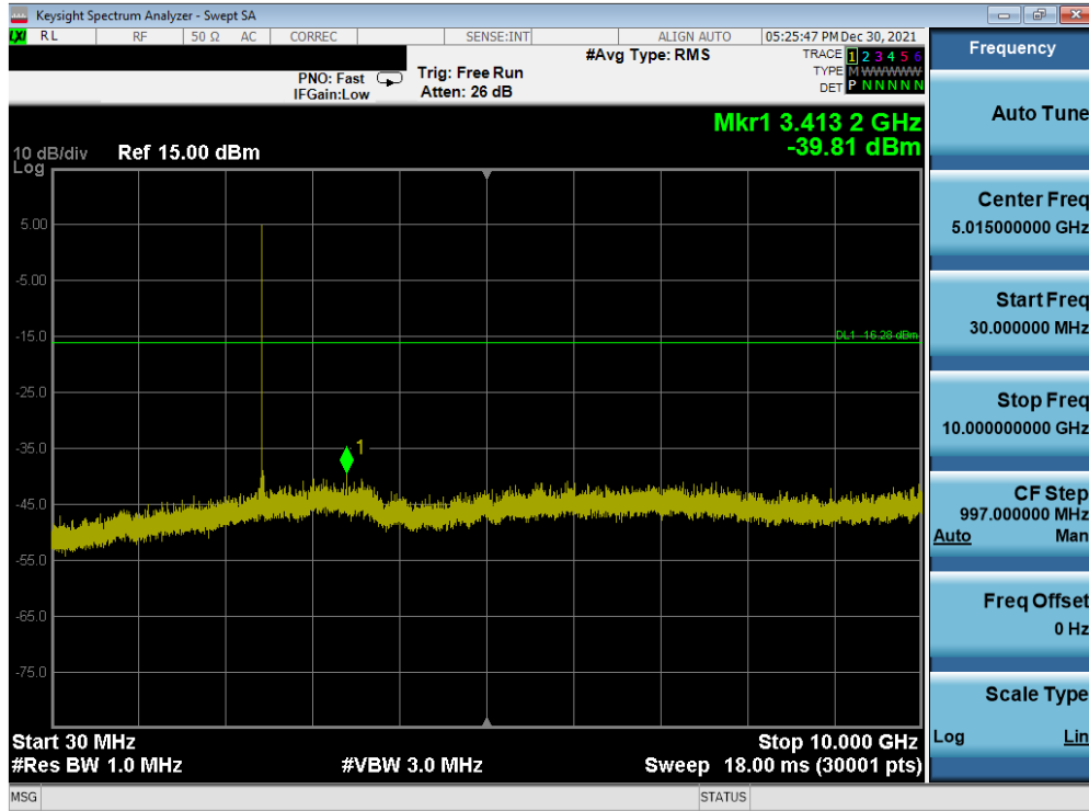
Plot 7-34. Conducted Spurious Plot (Bluetooth (LE), 1Mbps – Ch. 19)
