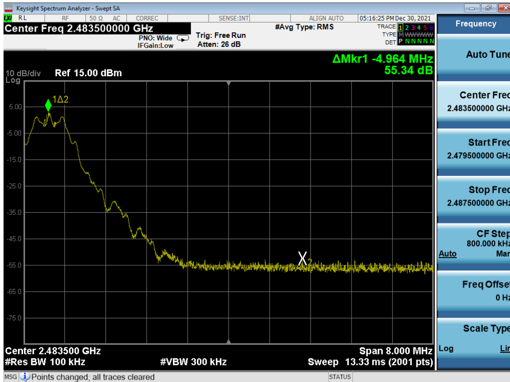
Plot 7-25. Band Edge Plot (Bluetooth (LE), 125kbps – Ch. 39)
