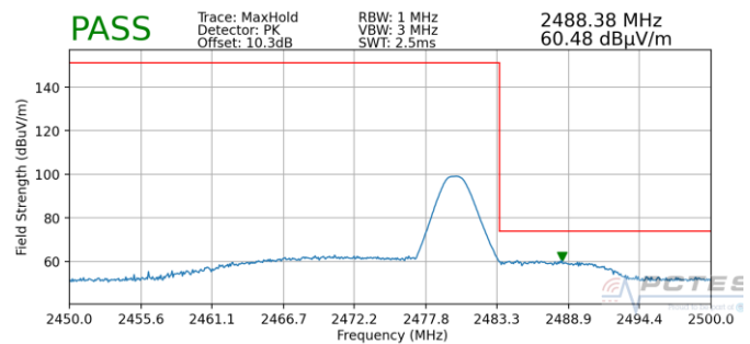
Plot 7-39. Radiated Restricted Upper Band Edge Measurement (Peak)
