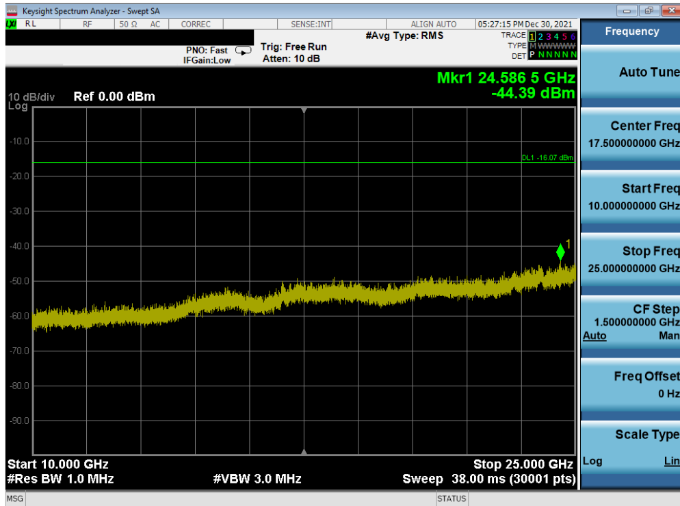
Plot 7-37. Conducted Spurious Plot (Bluetooth (LE), 1Mbps – Ch. 39)
