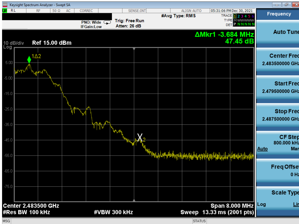
Plot 7-31. Band Edge Plot (Bluetooth (LE), 2Mbps – Ch. 39)
