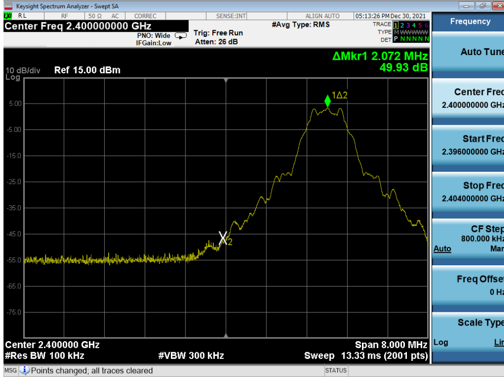
Plot 7-. Band Edge Plot (Bluetooth (LE), 125kbps – Ch. 0)
