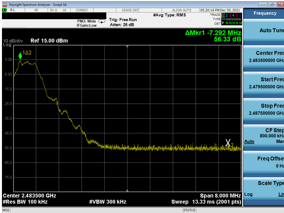
Plot 7-27. Band Edge Plot (Bluetooth (LE), 500kbps – Ch. 39)
