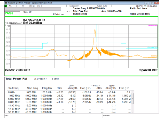
16QAM High channel 1RB_Offset High
