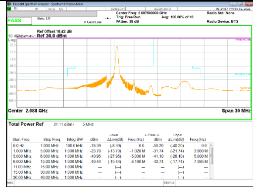
16QAM High channel 1RB_Offset Low
