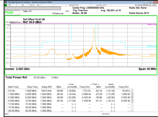
16QAM Mid channel 1RB_Offset High
