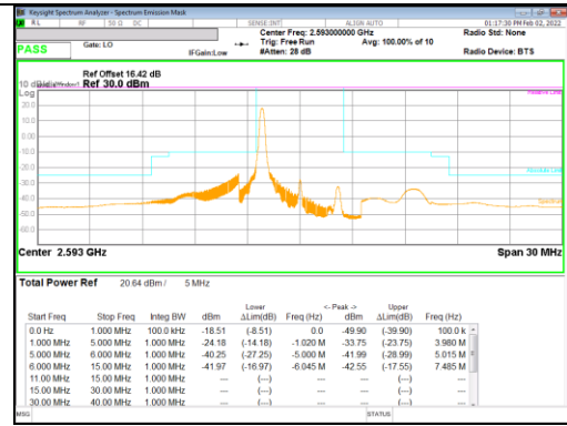
16QAM Mid channel 1RB_Offset Low
