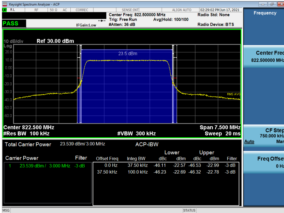
Plot 7-19. Channel - Ant1 Edge Plot (LTE Band 26 - 3MHz QPSK - High Channel)
