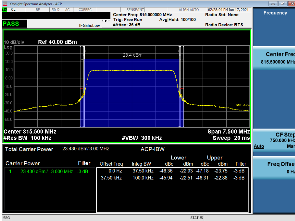
Plot 7-18. Channel - Ant1 Edge Plot (LTE Band 26 - 3MHz QPSK - Low Channel)
