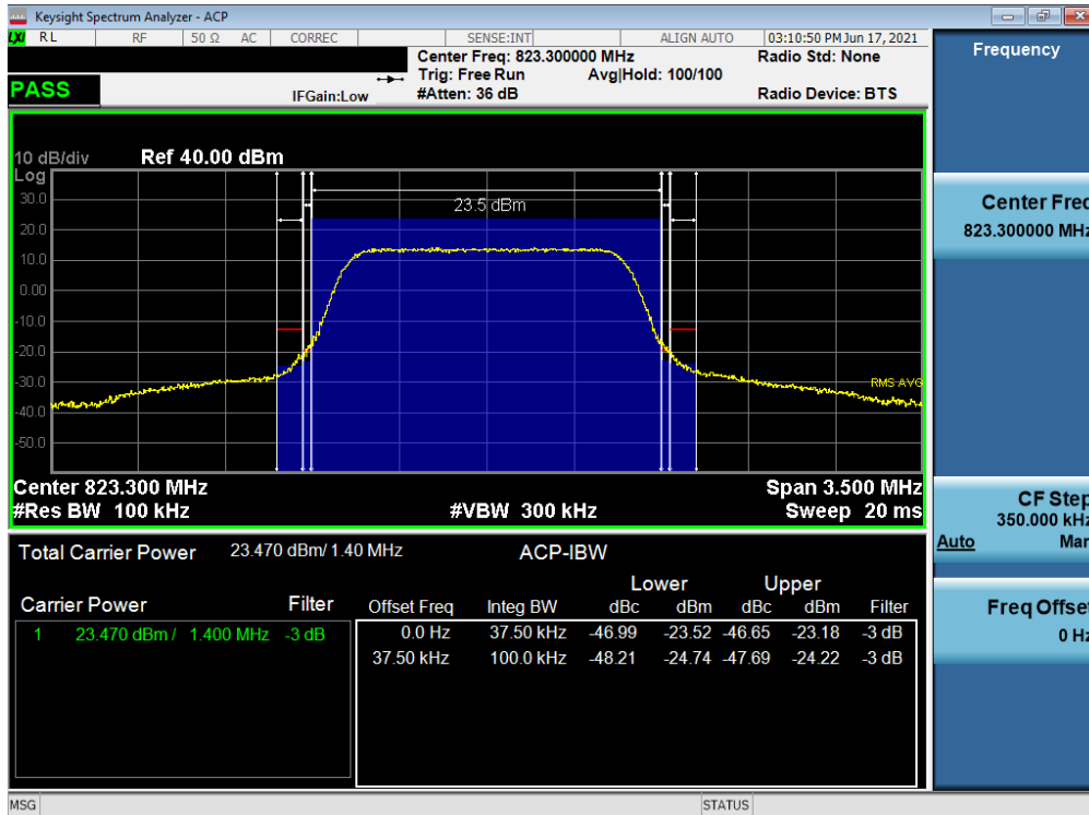
Plot 7-21. Channel - Ant1 Edge Plot (LTE Band 26 - 1.4MHz QPSK - High Channel)
