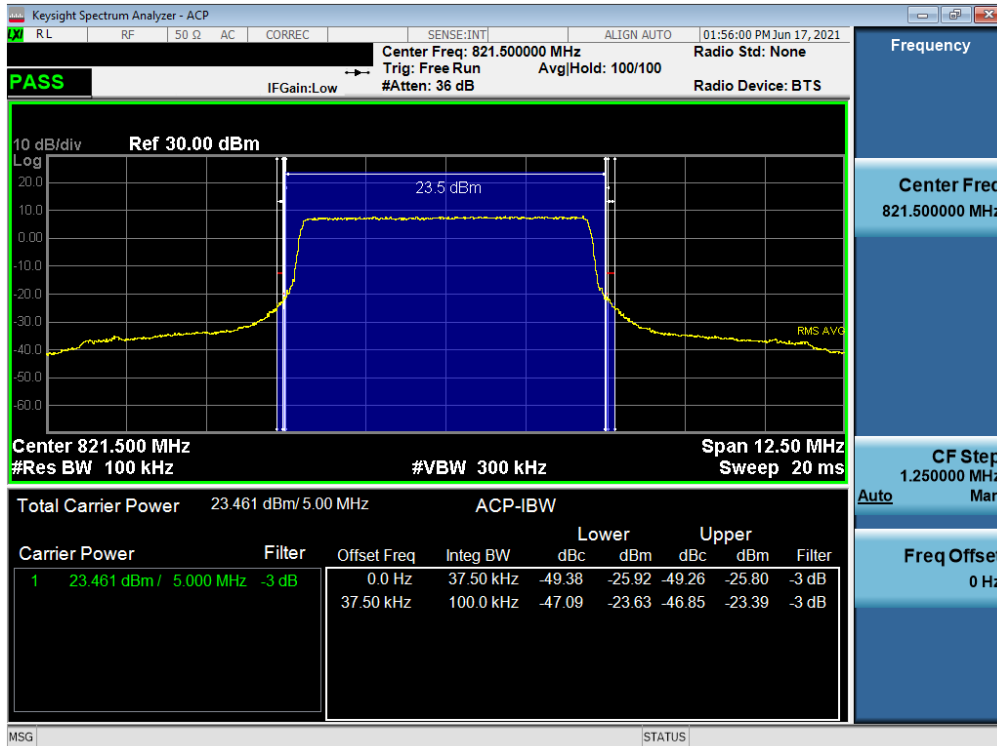
Plot 7-17. Channel - Ant1 Edge Plot (LTE Band 26 - 5MHz QPSK - High Channel)
