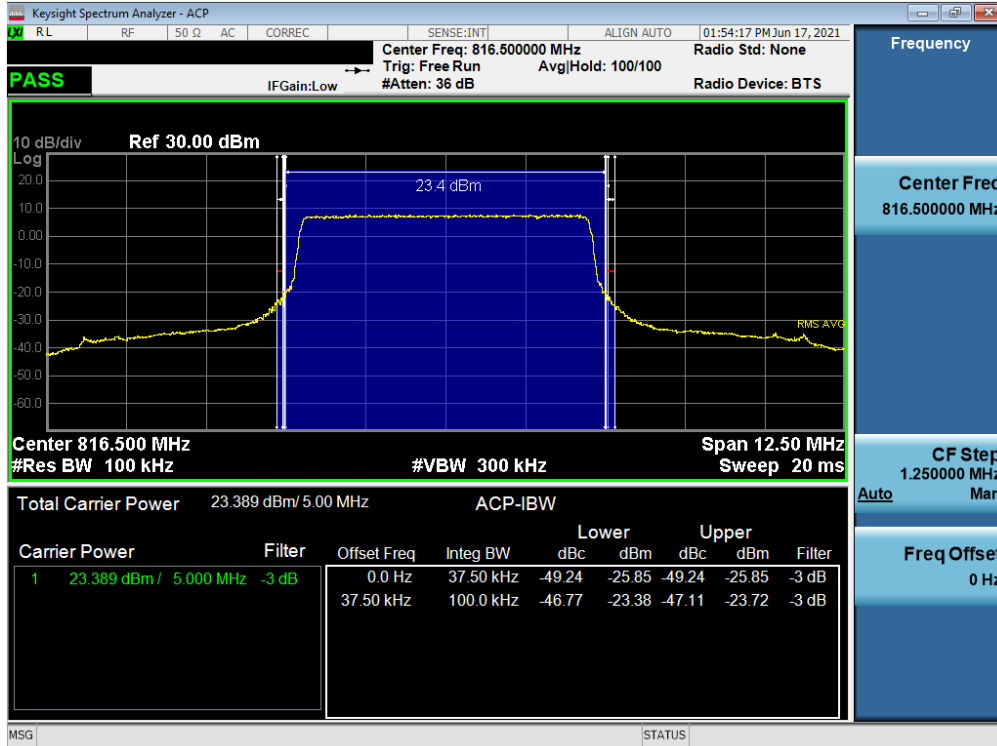
Plot 7-16. Channel - Ant1 Edge Plot (LTE Band 26 - 5MHz QPSK - Low Channel)
