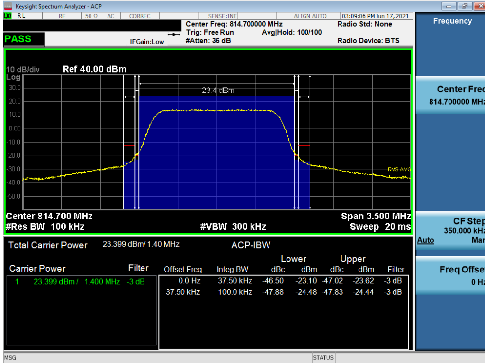
Plot 7-20. Channel - Ant1 Edge Plot (LTE Band 26 - 1.4MHz QPSK - Low Channel)
